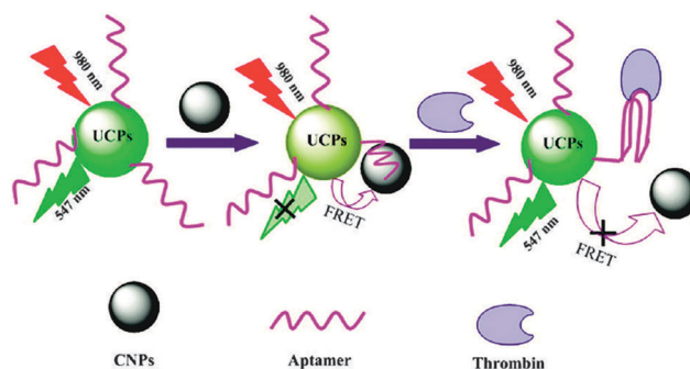
Fig. 17 Scheme of the design and function of a thrombin sensor based on UCNP. An aptamer on the UCNP surface binds to a carbon nanoparticle (CNP) via weak \pi - \pi interactions. The CNP quenches the upconversion emission by LRET. Thrombin changes the structure of the aptamer, releases the CNP from the UCNP surface and thus restores the upconversion emission. Reprinted with permission from ref. 38. Copyright © 2011, American Chemical Society.
