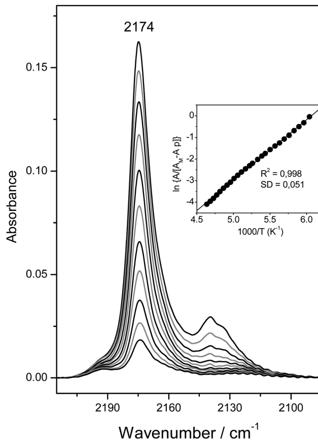
Fig. 6 Representative IR spectra (C–O stretching region) of CO adsorbed on H-MCM-22 (Si: Al = 24.5:1). From top to bottom, temperature goes from 154 to 214 K; and equilibrium pressure from 6.52 to 9.24 mbar. The inset shows the corresponding plot of the left-hand side of eqn (6) against the reciprocal of the temperature. R , linear regression coefficient; SD, standard deviation.
