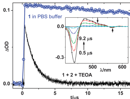
Fig. 4 Nanosecond transient absorption decay kinetics at 470 nm for { 1 + 2 + TEOA} (black) and { 1 in PBS} (blue) following 438 nm excitation. Inset: spectrum of { 1 + 2 + TEOA} at representative delay times 0.5, 0.8, 1.7, 4.1 and 9.2 \mu s (black, red, green, blue and cyan, respectively).
