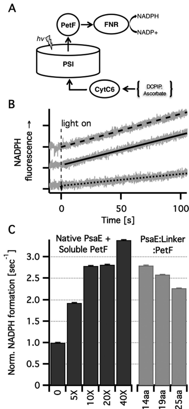
Fig. 4 In vitro light dependent \text{NADP}^+ reduction. (A) Scheme of the electron transport chain in solution. Photoexcited PSI was used to reduce PetF that carried the electrons to FNR where they were used for \text{NADP}^+ reduction to NADPH. Ascorbic acid was used as a sacrificial electron donor by reducing (via DCPIP) CytC6 that transferred the electrons to the oxidizing end of PSI. (B) NADPH formation rates were measured in vitro by monitoring the linear increase in NADPH fluorescence. Typical traces (grey lines) and their linear fits are shown for PSI with no PetF (dotted line), PSI with ten-fold PetF molar excess (dashed line) and PSI reconstituted with PsaE:19aa:PetF (solid line). (C) NADPH formation rates normalized by the rate for PSI reconstituted with native PsaE without PetF. Molar excess of soluble PetF to PSI are indicated. No PetF was added to the PSI complexes reconstituted with PsaE::PetF fusion proteins.
