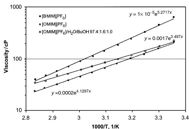
Fig. 1 Viscosity vs. 1/T .
