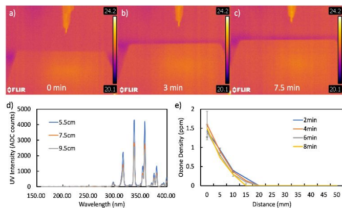
Fig. 5 Corona environmental impact: heat impact on the surface (a) before the corona is turned on, after corona treatment for (b) 3 minutes and (c) 7.5 minutes; (d) UV emission spectroscopy when the horizontal detection distance ranges from 5.5 cm to 9.5 cm away.
