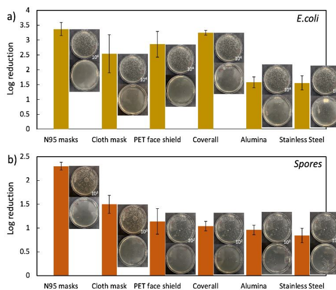
Fig. 2 The R of CD on different surfaces when contaminated with (a) E. coli and (b) G. stearothermophilus . The insets are images of the LB plates before and after CD treatment.
