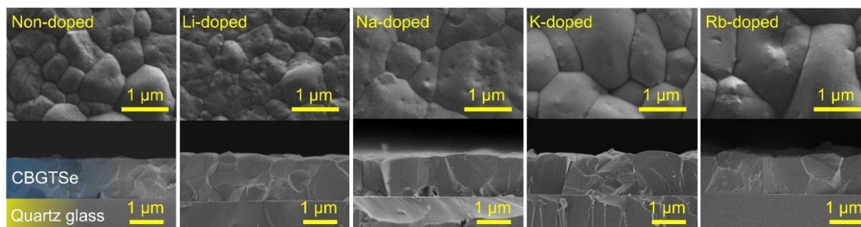
Fig. 1 Surface/cross-section SEM images for non-doped and alkali- (i.e. , Li, Na, K, and Rb) doped CBGTSe films deposited on quartz glass substrates. All scale bars represent 1 μm. Note that the alkali-doping was achieved by pre-depositing approximately 4 nm of alkali fluoride ( e.g. , KF) layers. Cross-section images were acquired after depositing ~5 nm of Au to avoid surface charging.
