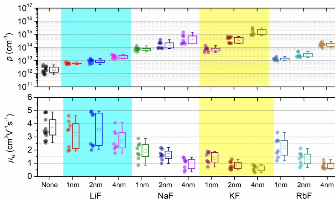
Fig. 4. Statistical distribution of the hole carrier densities ( \rho ) and Hall mobilities ( \mu_H ) extracted from Hall measurements on multiple (8–13) distinct non-doped and alkali-doped CBGTSe samples. The concentration of alkali content was controlled by varying the thickness of alkali fluoride layers ( i.e. , LiF, NaF, KF, and RbF) between 1 nm – 4 nm pre-deposited prior to CBGTSe films. The boxes are determined by (average) \pm (standard deviation), the “□” symbols represent the average values, and the horizontal lines correspond to the medians. Whiskers represent maximum and minimum data points.
