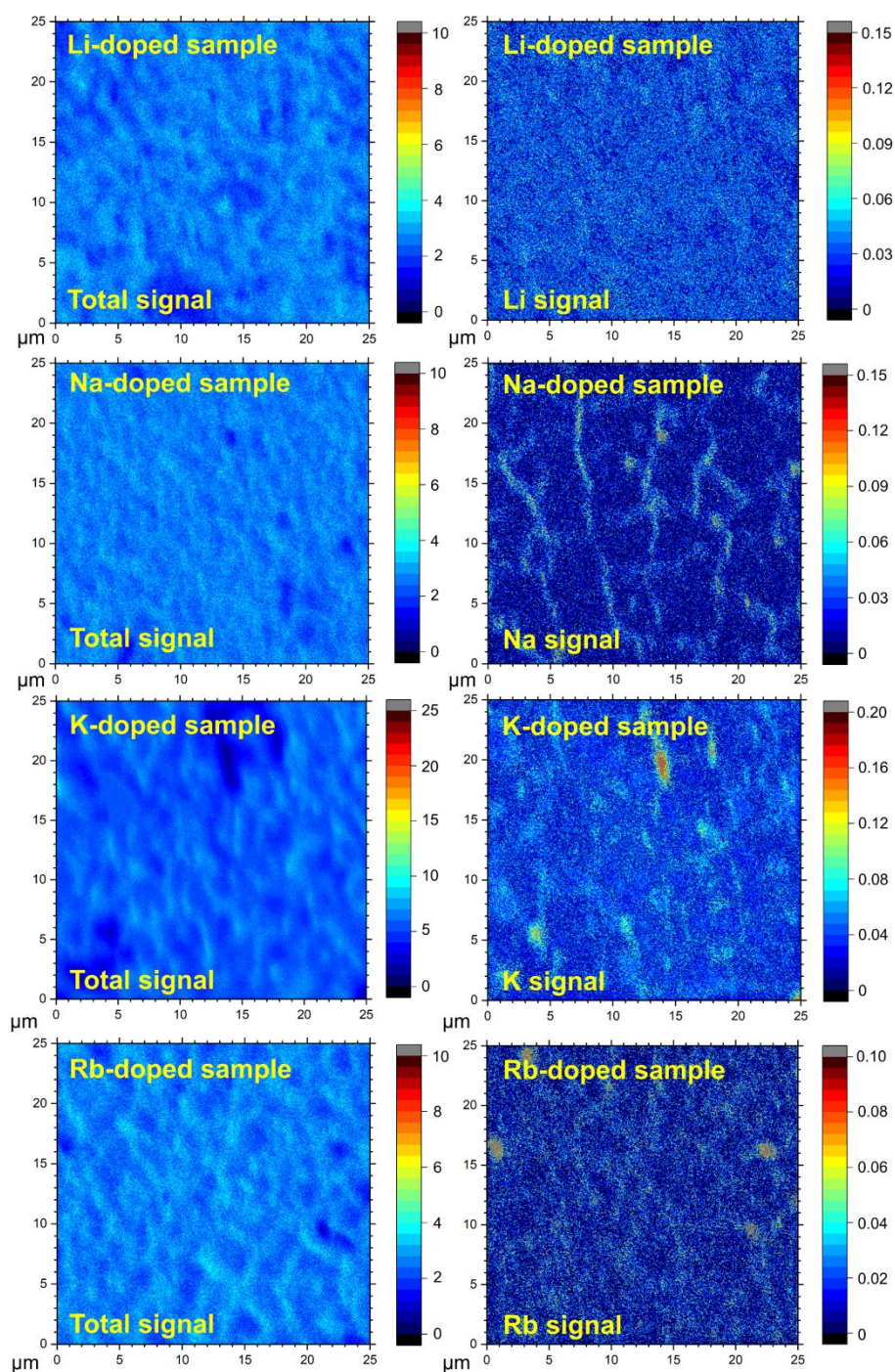
Fig. 3 TOF-SIMS 2D images for alkali-doped CBGTSe films prepared with pre-deposition of 4 nm alkali fluoride layer showing (left) total signal counts and (right) alkali-element signals. Each image was obtained by integrating the signals over 0.2–0.6 \mu\text{m} film depth. Alkali-element signals are normalized point-by-point to the total signal
