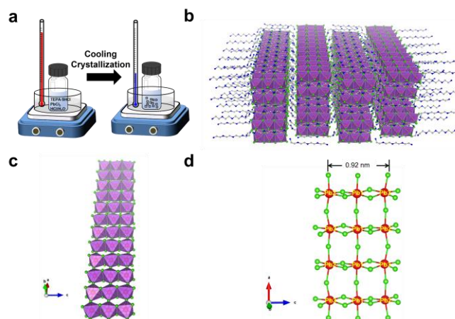
Figure 1. (a) Synthetic scheme for the material preparation; (b) crystal structure of C 8 H 28 N 5 Pb 3 Cl 11 (Grey spheres, carbon atoms; blue spheres, nitrogen atoms; red spheres, lead atoms; green spheres, chloride atoms; hydrogen atoms and oxygen atoms were hidden for clarity); (c) view of a lead chloride nanoribbon; (d) ball-and-stick model of a lead chloride nanoribbon.
