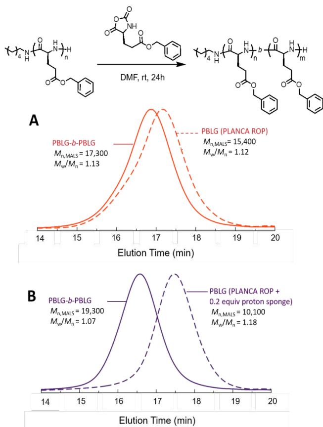
Figure 5. Chain-extension of A) PLANCA-derived PBLG (Table 1, entry 4 and 6), and B) PLANCA + PS-derived PBLG (Table 1, entry 5 and 7). Dashed line – PBLG, solid line – PBLG-b-PBLG
