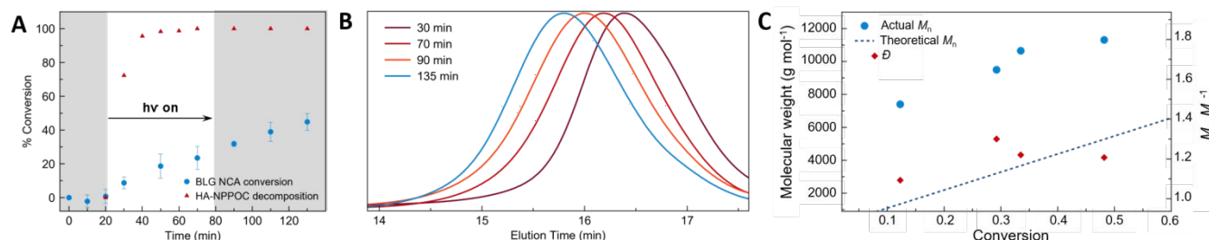
Figure 2. Photo-liberation of hexylamine (HA) from 2-(2-nitrophenyl)propyloxycarbonyl-protected HA (HA-NPPOC) for polymerization of \gamma -benzyl-L-glutamate (BLG): A) conversion versus time for the decomposition of HA-NPPOC and consumption of BLG NCA; B) SEC traces of kinetic aliquots, demonstrating increasing MW with time; C) experimental molecular weight (circles), theoretical molecular weight (dashed line), and molecular weight dispersity (diamonds) versus conversion. Molecular weights calculated from light scattering detection during SEC.
