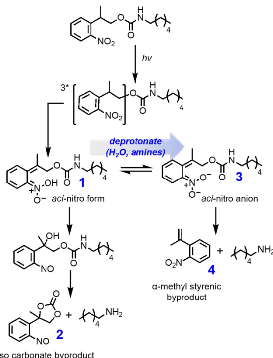
Figure 3. Photodeprotection of NPPOC-containing compounds proceeding through two different pathways to produce either a nitroso carbonate (2) or an \alpha -methyl styrenic byproduct (4).
