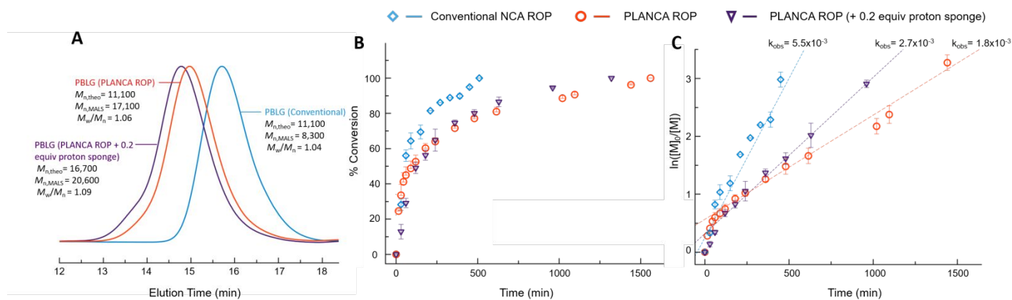
Figure 4. A) SEC traces at full monomer conversion, B) monomer conversion versus time, and C) pseudo-first-order kinetic plots for conventional NCA ROP, PLANCA ROP, and PLANCA ROP with 0.2 equiv of proton sponge. Molecular weights calculated from light scattering detection during SEC.
