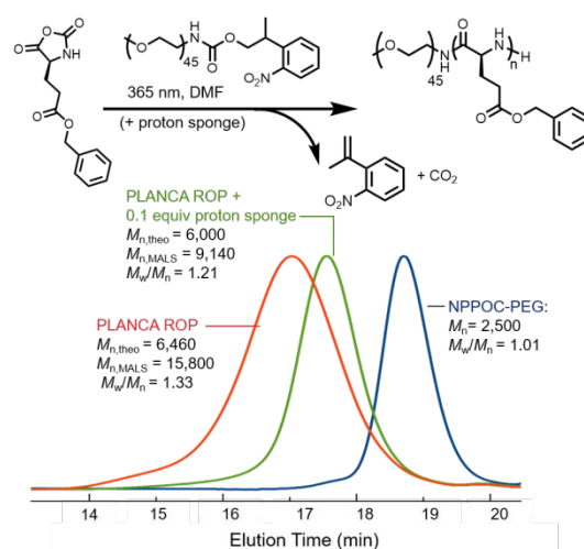
Figure 6. Synthesis of polypeptide block copolymers by light, using PLANCA ROP with NPPOC-protected PEG-amine. Molecular weights determined from light scattering detection during SEC.
