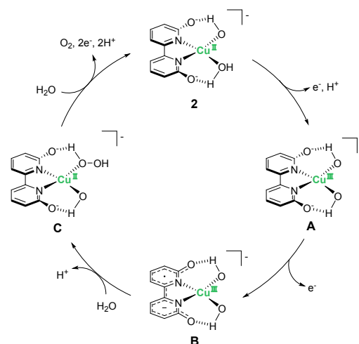
Figure 2. Plausible catalytic cycle for the water oxidation reaction mediated by Copper-bipyridine complex 2 .
