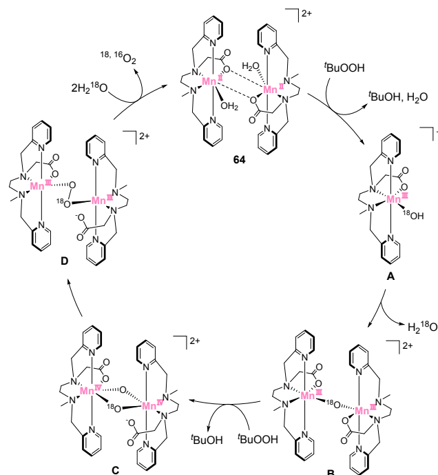
Figure 29. Catalytic cycle for water oxidation by the manganese dimer complex with a monoanionic pentadentate ligand 64 initially proposed by McKenzie et al.
