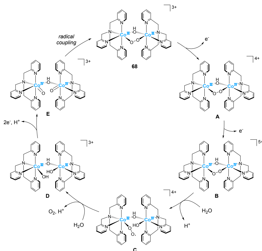
Figure 32. Proposed mechanism for water oxidation promoted by the \mu -O 2 bridged cobalt dimer complex 68 .
