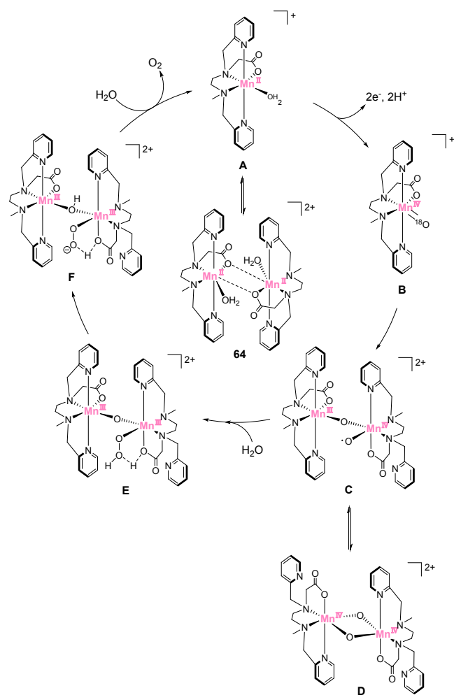
Figure 30. Updated catalytic mechanism for water oxidation mediated by 64 reported in 2011.
