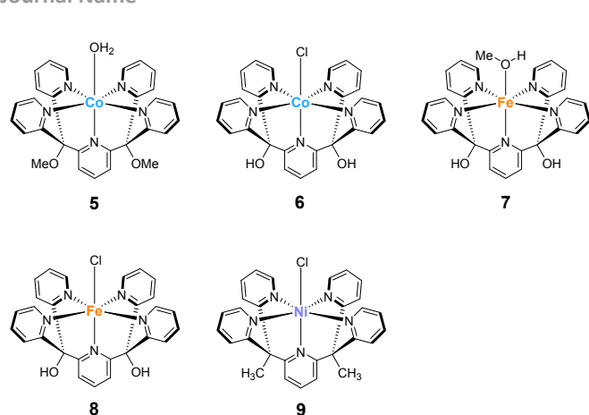
Chart 4. Structures of mononuclear water oxidation catalysts with PYS-type ligands.
