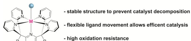
Chart 5. Summary of features of water oxidation catalysts with PY5-type ligands.
