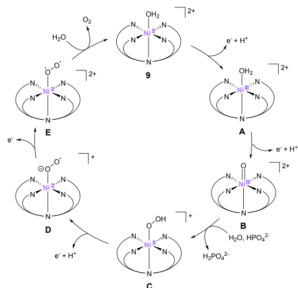
Figure 8. Proposed mechanism for electrocatalytic water oxidation by Ni-PY5Me complex 9 .
