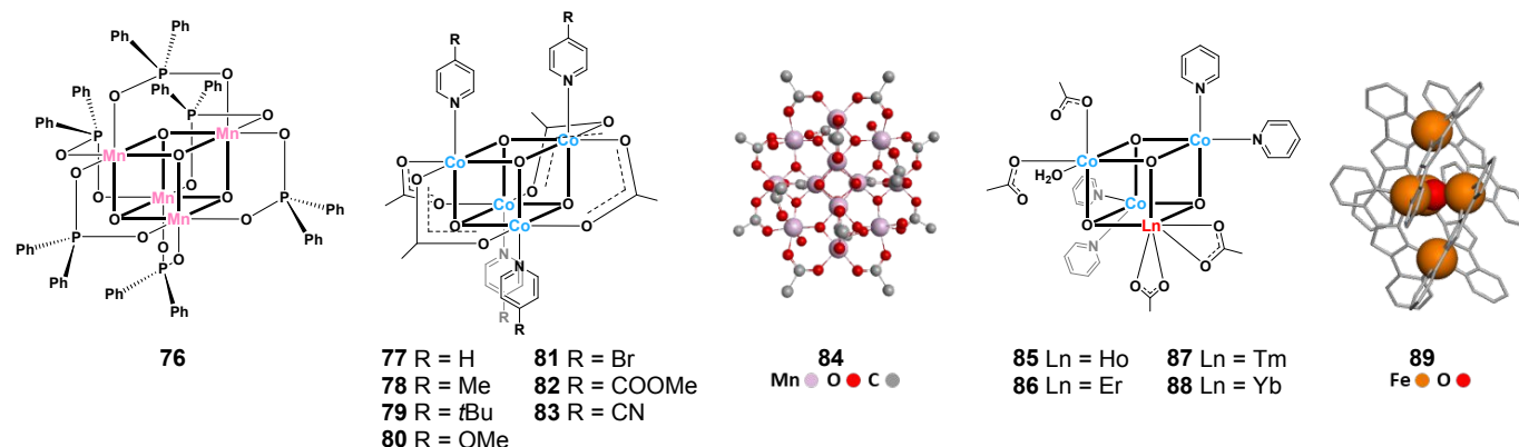
Chart 14. Structures of multinuclear water oxidation catalysts.
