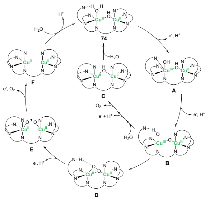
Figure 36. Proposed mechanism of water oxidation catalysed by the dimeric copper complex 74 , which operates in neutral aqueous solutions.
