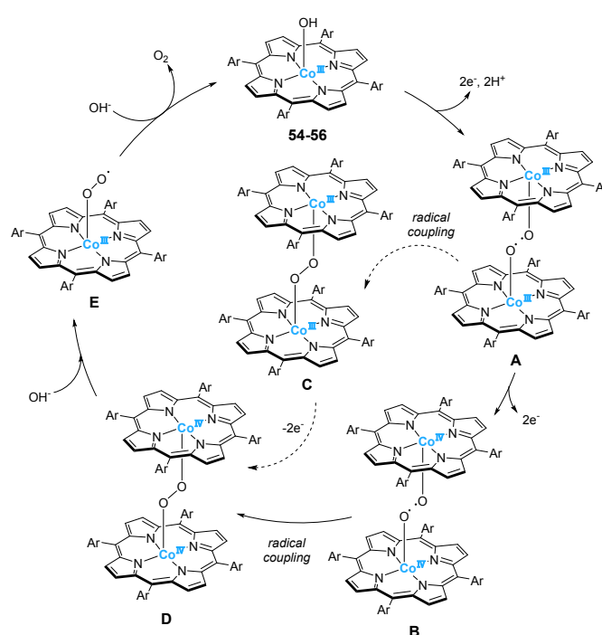
Figure 24. Plausible reaction mechanism of photocatalytic water oxidation by the water-soluble cobalt-porphyrin complexes 54–56 .
