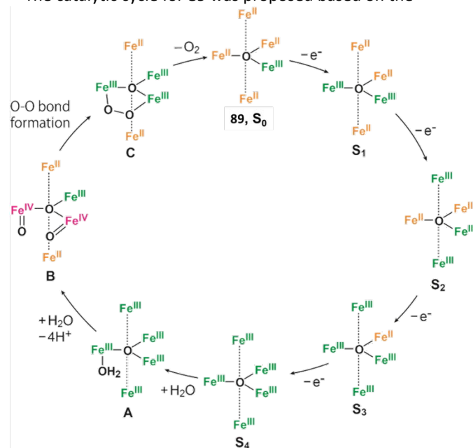
Figure 40. Plausible catalytic cycle water oxidation promoted by the pentanuclear iron complex 89 .
