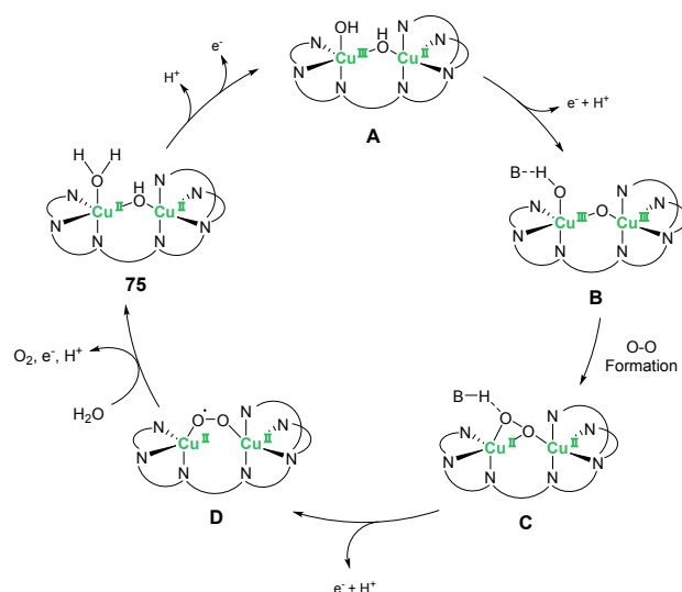
Figure 37. Proposed mechanism for water oxidation by the unsymmetrical dimeric copper complex 75 .
