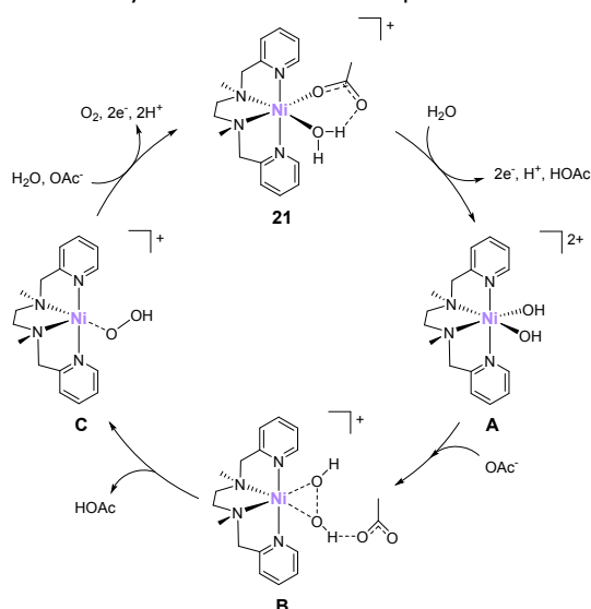
Figure 11. Proposed pathway for water oxidation by Ni-PY5 complex 21 in phosphate buffer solution.
