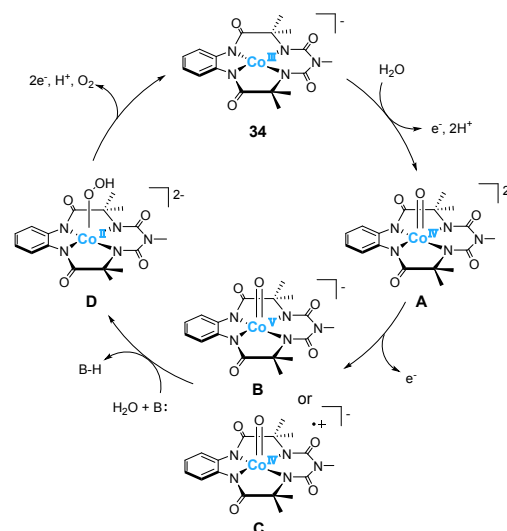
Figure 16. Proposed catalytic mechanism of the cobalt complex bearing the biuret-modified TAML (bTAML) ligand 34 .
