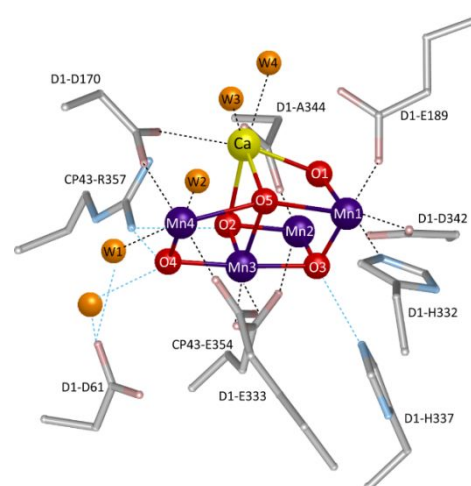
Figure 38. The structure of the \text{Mn}_4\text{CaO}_5 cluster and its ligand environment in the OEC. Manganese, purple; calcium, yellow; oxygen, red; oxygen atoms in water molecules, orange. Most intensively investigated. Development of such complexes is an interesting research target because such studies can contribute both to the understanding of the features of the OEC, and the construction of artificial water oxidation catalysts. However, most of the structural models of the OEC are inactive
