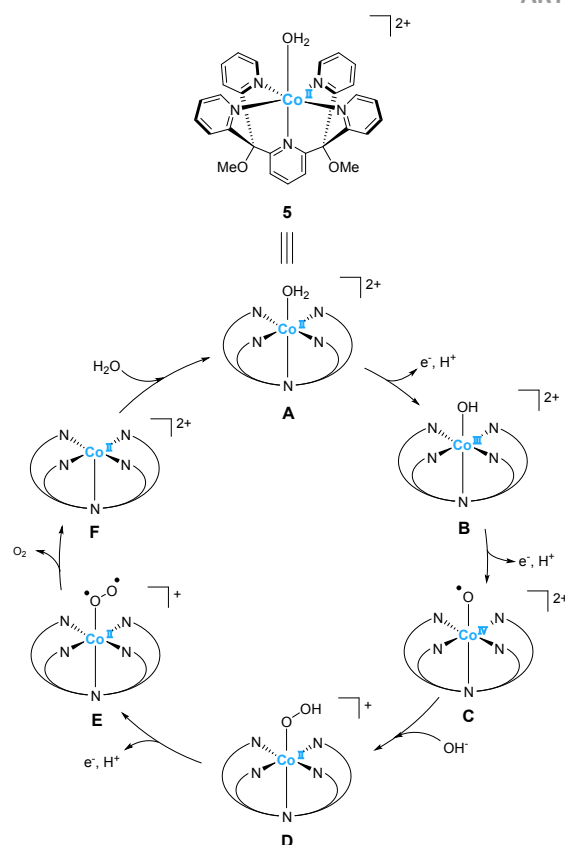
Figure 4. Proposed water-oxidation mechanism using Co-PYS complex 5 as a catalyst.
