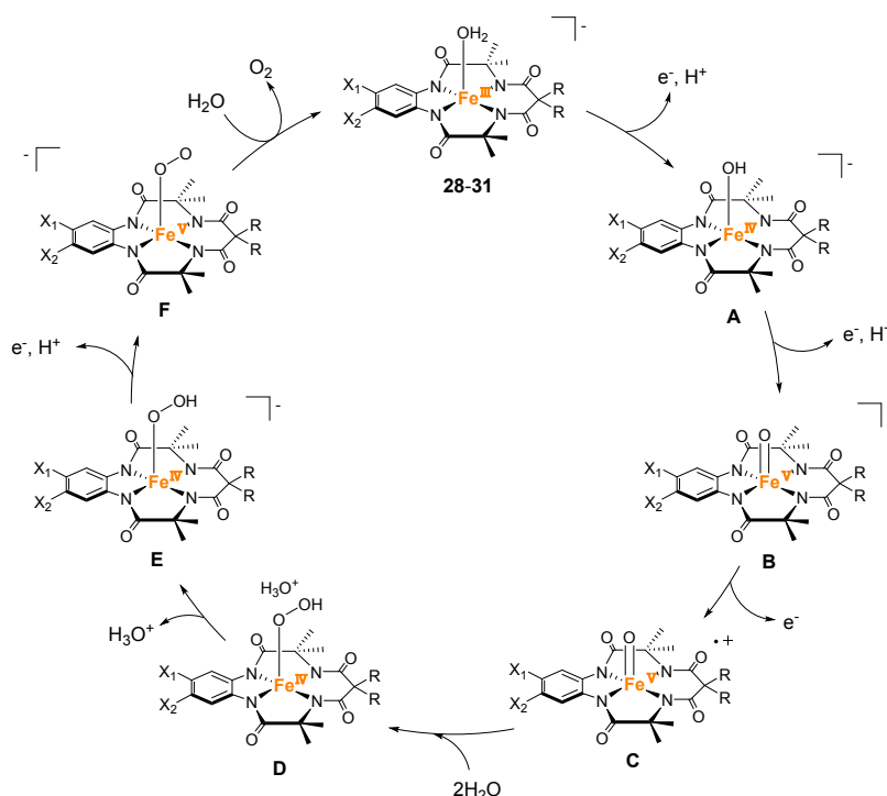
Figure 14. Proposed pathway for water oxidation with iron complexes bearing the tetra-amido macrocyclic ligands (TAMLs) 28-31 .
