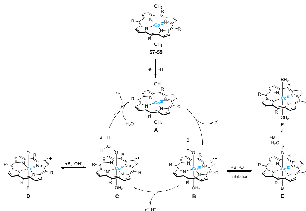
Figure 25. Plausible catalytic cycle of water oxidation promoted by the water-soluble cationic cobalt porphyrins 57-59.
