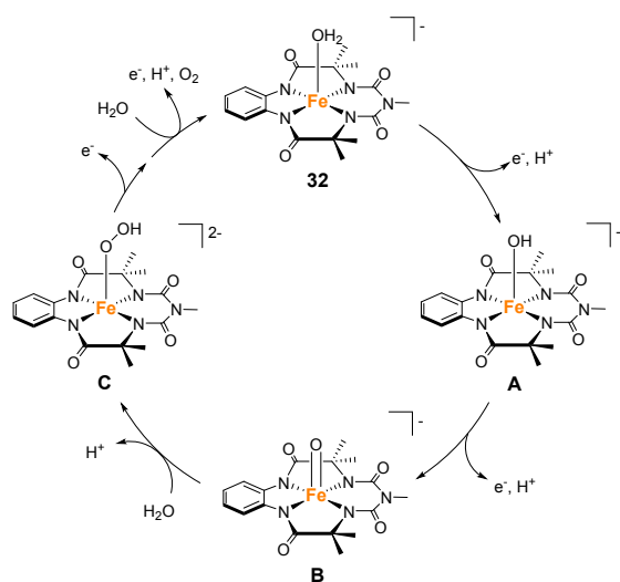
Figure 15. Proposed water oxidation mechanism of the iron complex with biuret-modified tetra-amidomacrocyclic ligand 32 .
