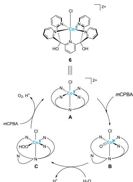
Figure 5. Postulated mechanism for water oxidation by Co-PY5OH complex 6.
