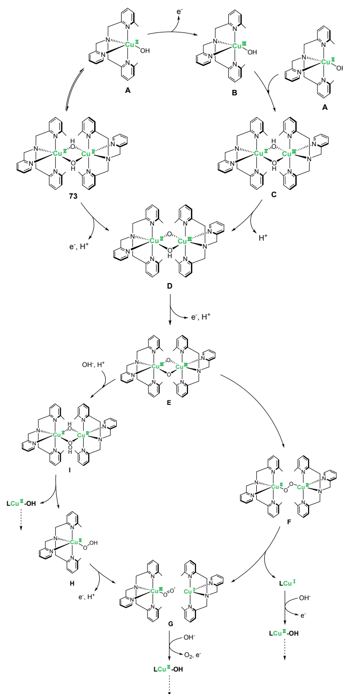
Figure 35. Plausible catalytic mechanism for water oxidation by the copper-based dimeric complex 73
