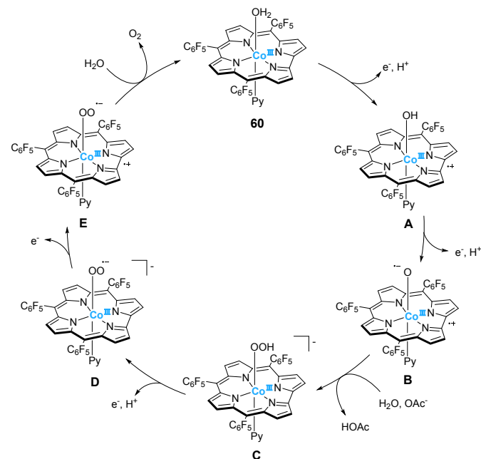
Figure 26. Proposed mechanism for water oxidation mediated by the cobalt-based corrole complex 60 .
