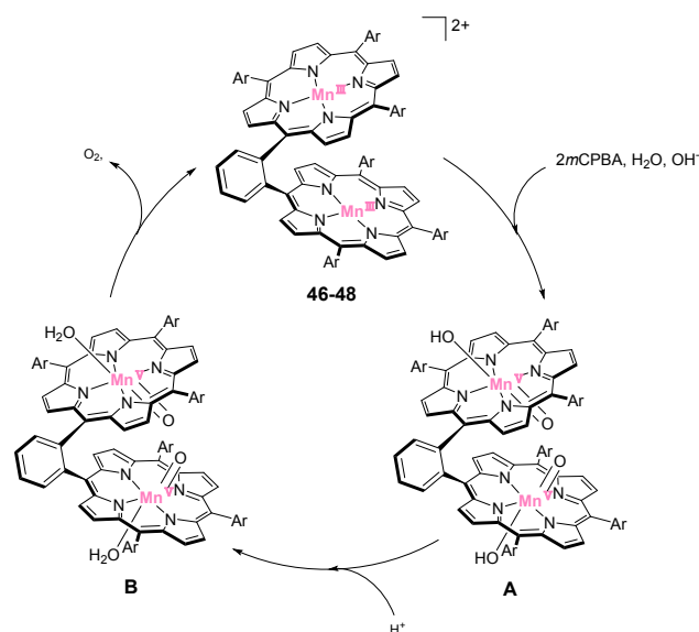
Figure 22. Proposed catalytic cycle of water oxidation promoted by Mn-based bis-porphyrin complexes 46–48 .
