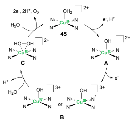
Figure 21. Plausible catalytic cycle for water oxidation mediated by the copper-based complex with TMC ligand 45 .
