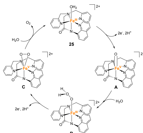
Figure 13. Proposed catalytic cycle for the water oxidation reaction by the iron complex with an anionic pentadentate alkylamine pyridyl-type ligand 25 .
