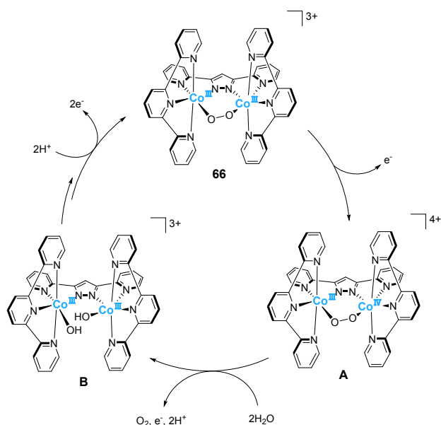
Figure 31. Plausible catalytic pathway of water oxidation mediated by the \mu -peroxo cobalt dimeric complex 66 .
