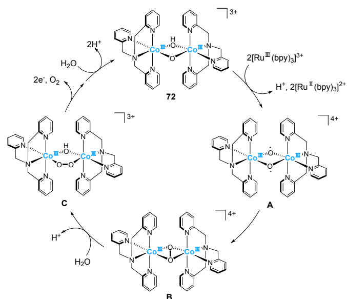
Figure 34. Possible catalytic pathway for water oxidation mediated by the dinuclear cobalt complex 72 .
