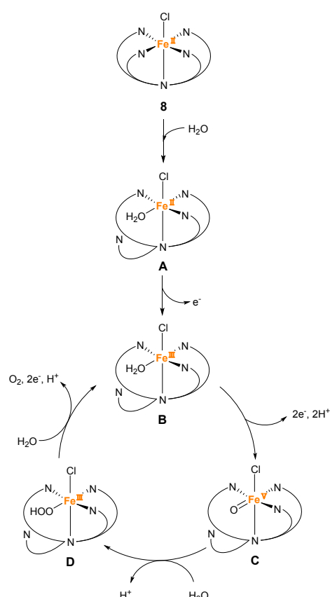
Figure 7. Proposed mechanism for water oxidation by Fe-PY5OH complex 8 using [\text{Ru}(\text{bpy})_3]^{3+} as a chemical oxidant.
