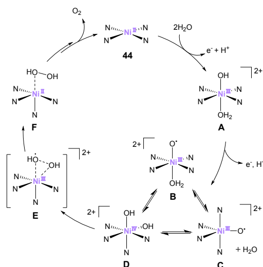
Figure 20. Proposed mechanism for water oxidation by the nickel complex with 1,4,8,11-tetramethyl-1,4,8,11-tetraazacyclotetradecane (TMC)-type ligand 44 .
