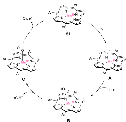
Figure 23. Plausible catalytic pathway of water oxidation by the manganese-based corrole complex 51 .
