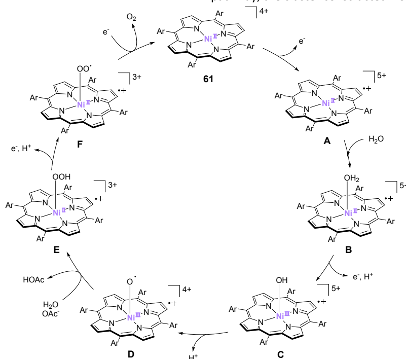
Figure 27. Plausible catalytic cycle for water oxidation facilitated by the water-soluble Ni-porphyrin complex 61 .
