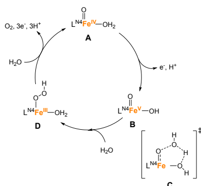
Figure 9. Postulated mechanism for water oxidation by iron Complexes 10-14 based on tetradentate nitrogen ligands.
