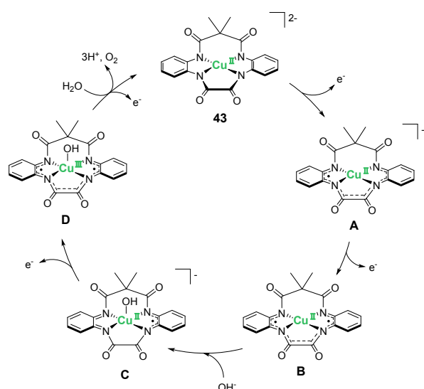
Figure 19. Proposed mechanism for water oxidation promoted by the copper-based TAML complex 43 .
