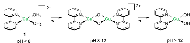
Figure 1. The acid-base equilibrium of 1 in solution at different pH values.
