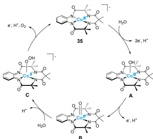
Figure 17. Proposed mechanism for water oxidation mediated by the Co-TAML complex 35 .
