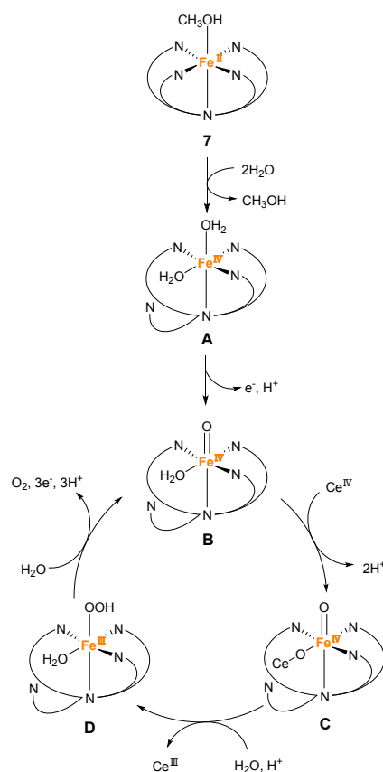
Figure 6. Proposed mechanism for water oxidation by Fe-PY5OH complex 7 using CAN as a chemical oxidant.
