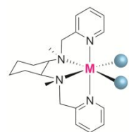
Chart 7. Summary of features of water oxidation catalysts with alkylamine-pyridine ligands.
