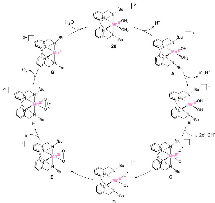
Figure 10. Proposed catalytic cycle for water oxidation mediated by Manganese pyridinophane complex 20 .
