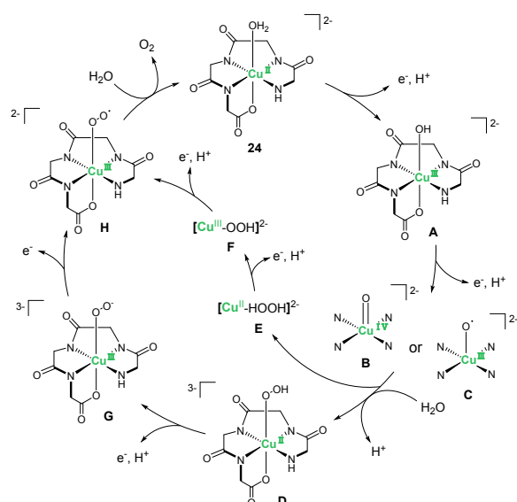
Figure 12. Proposed mechanism for water oxidation mediated by the copper complex bearing the polypeptide ligand 24 .
