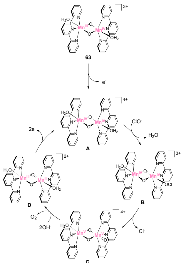
Figure 28. Plausible catalytic pathway for water oxidation mediated by the bis( \mu -O)-bridged dinuclear manganese complex 63
