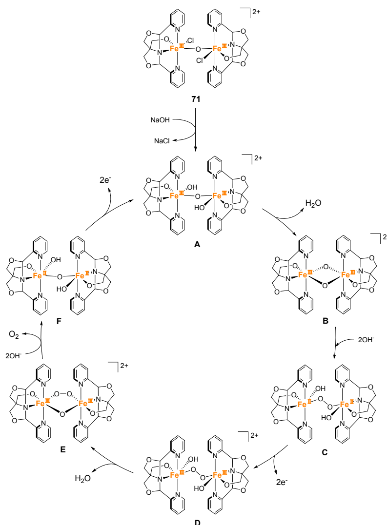
Figure 33. Plausible catalytic mechanism for water oxidation mediated by 71 .
