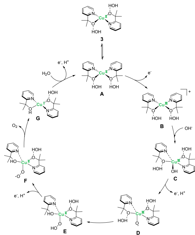
Figure 3. Catalytic cycle for water oxidation with the Copper-PyalkH complex 3 .
