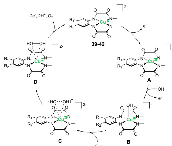
Figure 18. Plausible catalytic pathway of water oxidation promoted by the copper-based complexes with TAML-like ligands 39–42 .
