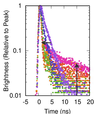
Fig. 8 Time resolved photoluminescence of the ( w:(0:5:1) ) copolymer at 520 nm. As in Fig. 6, the sensitizer is quenched (arrow towards left) by the formation of a long-lived excimer (upwards arrow).
