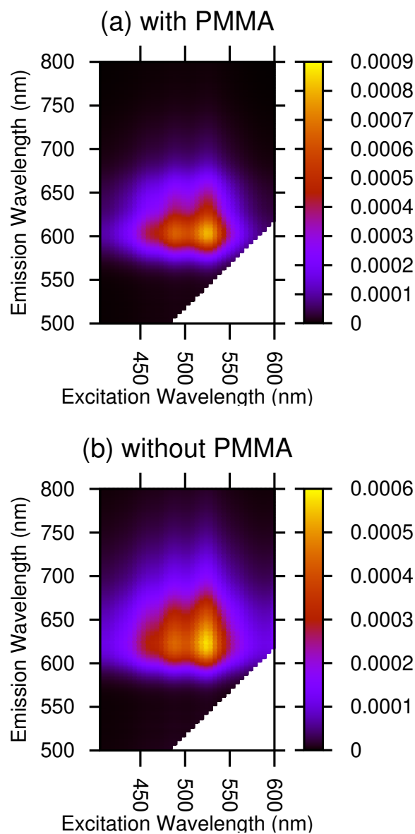
Fig. 13 Model of the contribution of energy transfer to excitation-emission, with (a) and without (b) PMMA.
