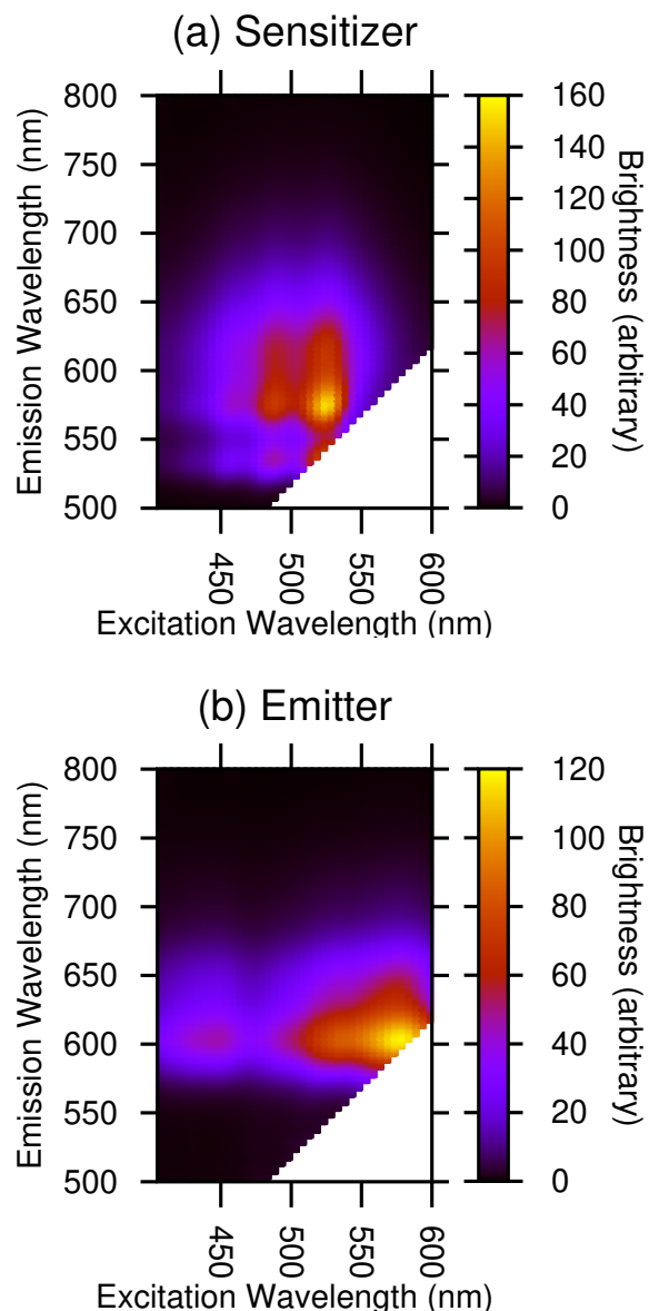
Fig. 12 Excitation-emission spectra of the sensitizer 0.7k:(5:1:0) (a) and emitter 1.9k:(20:0:1) (b). The emitter emission occurs and longer wavelengths than the sensitizer absorption, indicating suitability of the system for solar concentration. The white region shows where data was removed because the excitation wavelength was not substantially less than the emission wavelength.
