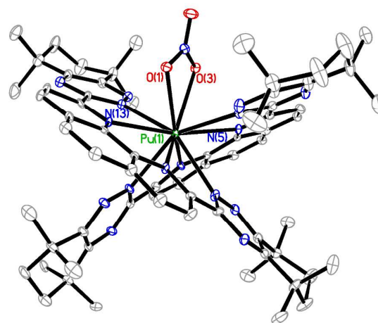
Figure 2. Thermal ellipsoid plot of the solid-state structure of [Pu III (CyMe 4 -BTPhen) 2 (NO 3 )][Pu IV (NO 3 ) 6 ] 2 ·4MeCN. The [Pu IV (NO 3 ) 6 ] 2- anion, lattice solvent, and H atoms have been omitted for clarity.
