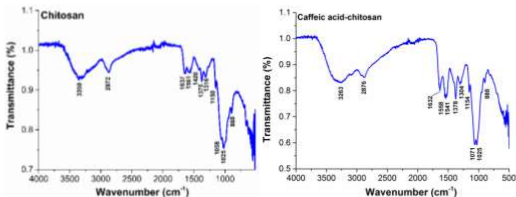
Fig. 3 FT-IR spectra of chitosan and chitosan-caffeic acid
