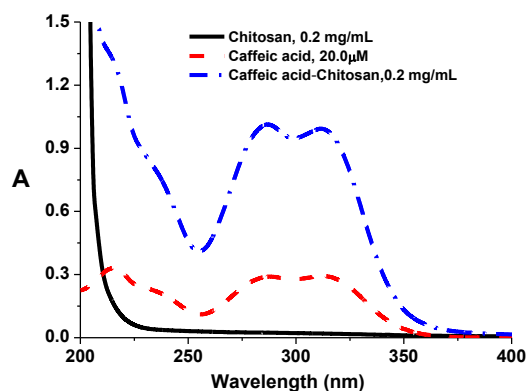
Fig. 1 UV spectra of chitosan (0.2 mg/mL), caffeic acid (20 μM), chitosan-caffeic acid (0.2 mg/mL) in 18 mΩ·cm water, T = 298 K.
