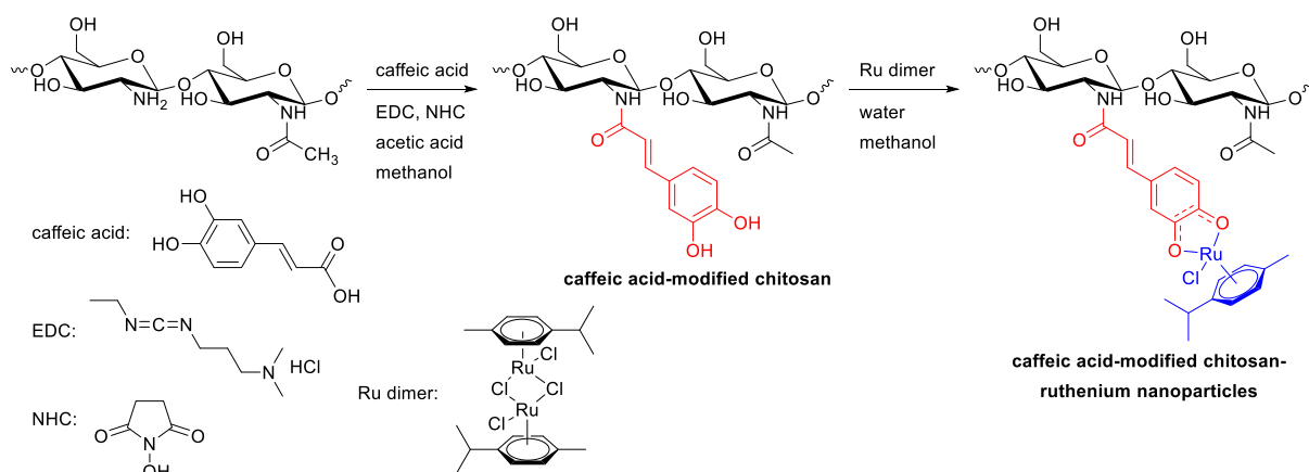
Scheme 1. Synthetic route for caffeic acid-modified chitosan-ruthenium nanoparticles
