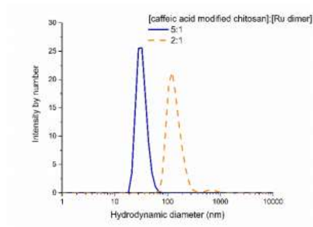
Fig. 7 Dynamic light scattering of Ru-caffeic acid modified chitosan at two different ratios.
