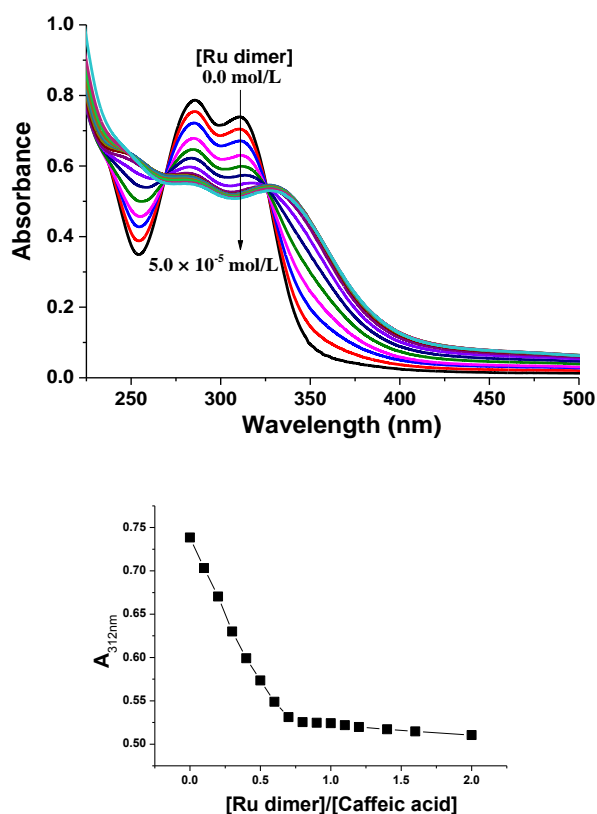
Fig. 6. Top: UV-vis spectra for the reaction of various concentrations of Ru dimer with caffeic acid-modified chitosan, [\text{caffeic acid in caffeic acid-modified chitosan}] = 5.0 \times 10^{-5}
