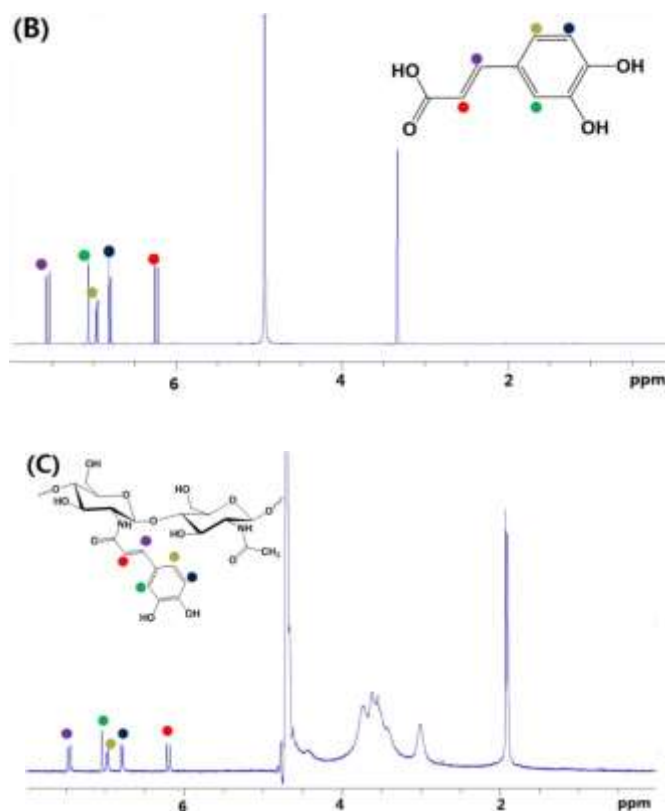
Fig. 2. 1 H NMR spectra of (A) chitosan in 1% CD 3 COOD in D 2 O, (B) caffeic acid in CD 3 OD, and (C) chitosan-caffeic acid in D 2 O.
