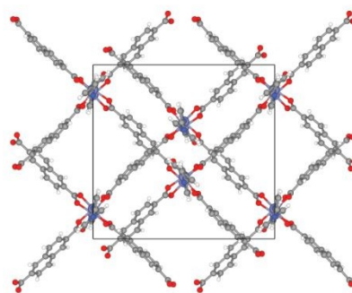
CSD refcode: RELAW (Zn, pcu )
