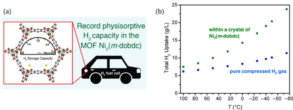
Fig. 9 (a) Schematic illustration of the physisorptive \text{H}_2 capacity in \text{Ni}_2(m\text{-dobdc}) and (b) comparison of total volumetric capacities and pure compressed \text{H}_2 of \text{Ni}_2(m\text{-dobdc}) at 100 bar 147 (reproduced from ref. 147 with permission from The American Chemical Society, copyright 2018).
