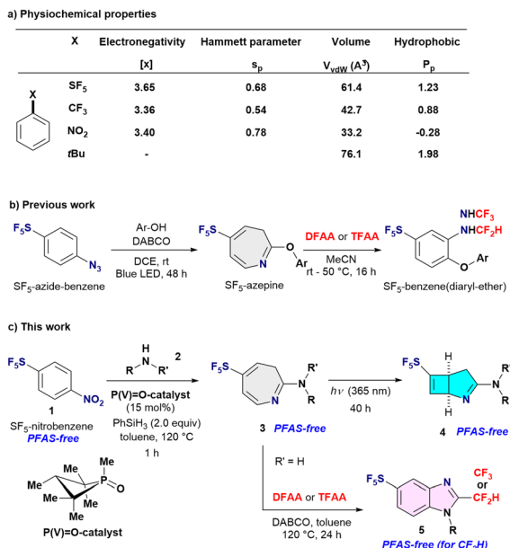
Fig. 1 Background of this work. (a) Properties of SF 5 vs. CF 3 , NO 2 and tBu-benzenes. (b) Previous work (c) This work.
