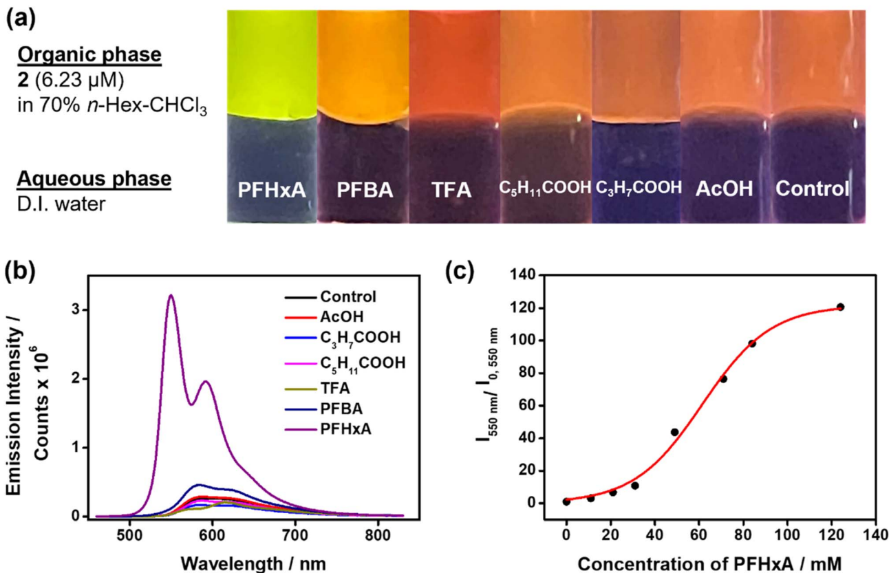
Fig. 5 (a) Photographs under a UV-light source ( \lambda_{\text{ex}} = 365 \text{ nm} ) and (b) emission spectra of 2 in 70% n -hexane- \text{CHCl}_3 ( 6.23 \mu\text{M} , 2 mL) after extraction with various species in deionized water (125 mM, 2 mL). The excitation wavelength is 425 nm. (c) A plot of relative emission intensity at 550 nm against initial concentration of PFHxA in the aqueous phase.
