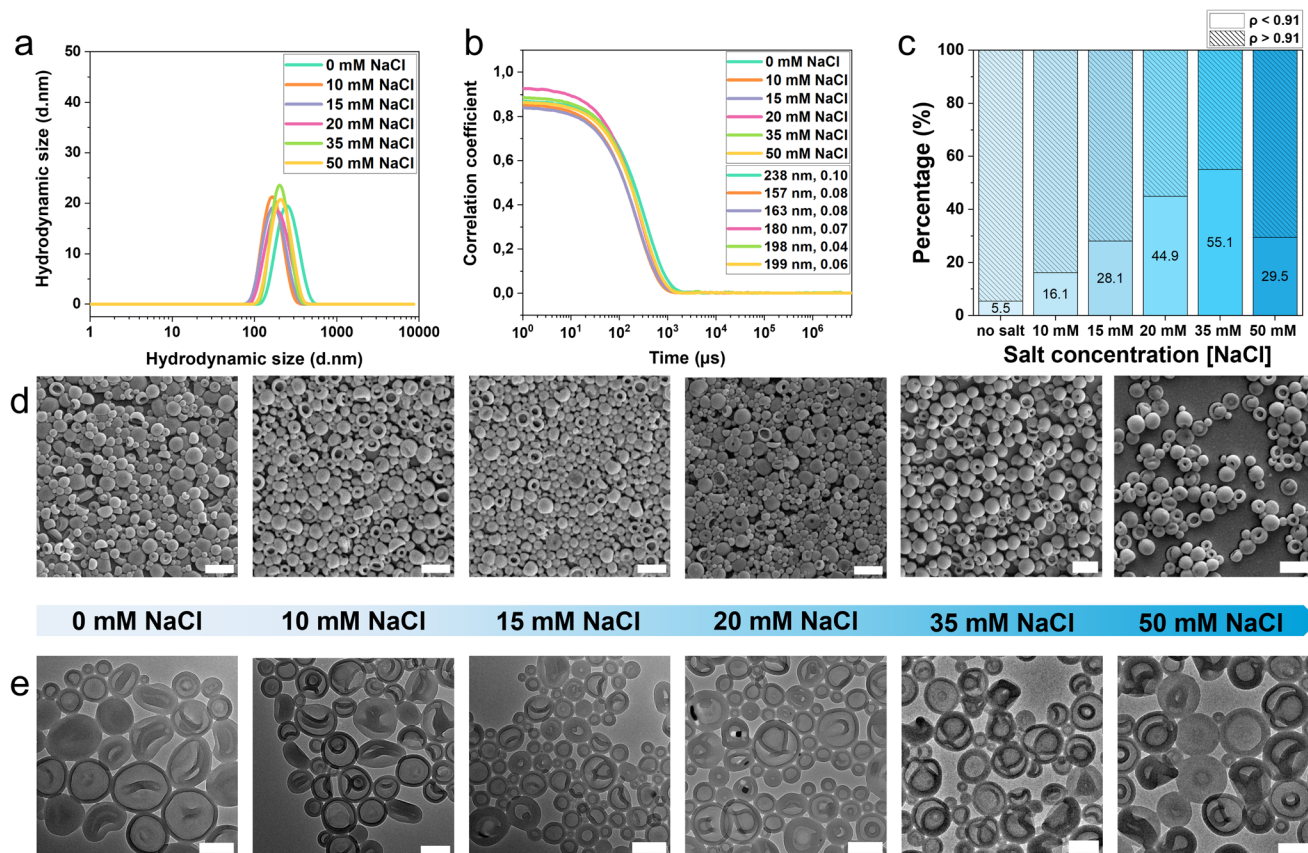
Fig. 3 Effect of NaCl concentration on the assembly of polymer P1: A-(B-C)/0.06 and the subsequent shape transformation. (a) Dynamic light scattering size-intensity comparison, (b) correlogram displaying hydrodynamic diameter and PDI, (c) distribution analysis of polymeric vesicles calculated from AF4 data, displaying the percentage of stomatocytes. (d) SEM and (e) TEM images of the samples prepared with different salt concentrations. SEM scale bar = 500 nm, TEM scale bar = 200 nm.
