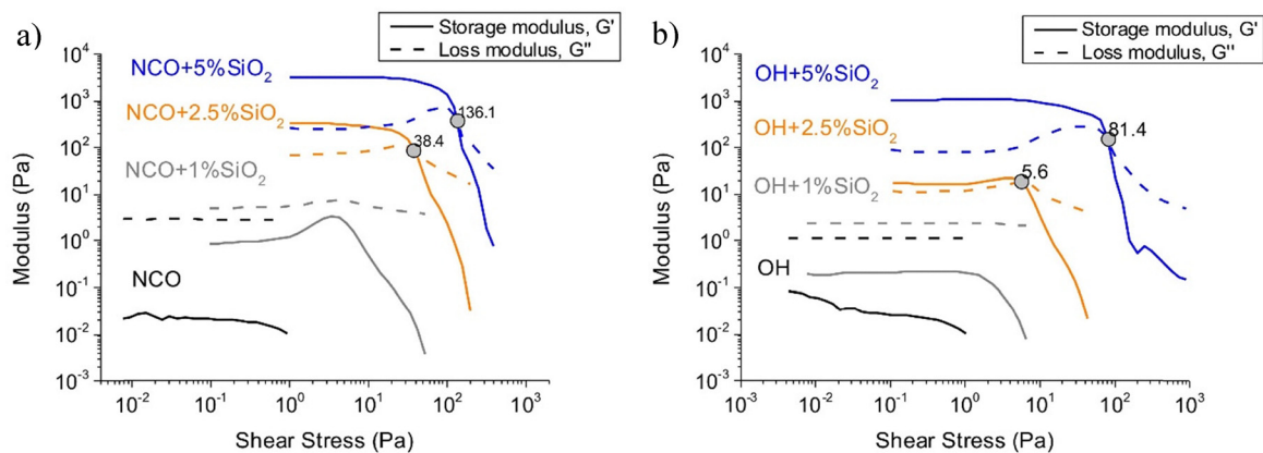
Fig. 3 Oscillatory rheology data of the investigated feeds showing a plot of modulus versus shear stress for the (a) isocyanates (NCO) and (b) polyol (OH) feeds.
