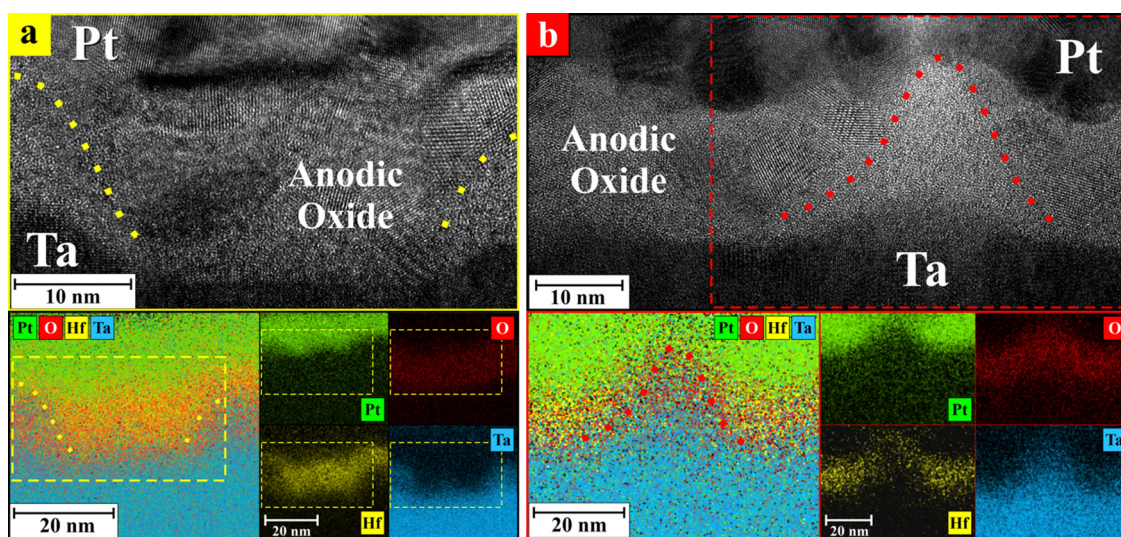
Fig. 4 Composite \text{Hf}/\text{Ta} oxides of anodic memristors grown (a) in citrate buffer and (b) in phosphate buffer together with the correspondent elemental energy-dispersive X-ray spectroscopy maps. The approximate position of the amorphous \text{Ta}_2\text{O}_5 nanocolumns surrounded by the polycrystalline \text{HfO}_2 matrix is highlighted with dotted lines. 48
