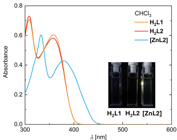
Fig. 3 UV-vis spectra recorded of H 2 L1 (orange), H 2 L2 (red), and of the zinc(II) reference complex [ZnL2] (blue) in \text{CHCl}_3 solutions ( c_0 \approx 3 \times 10^{-5} M). Inset: Photo of the solutions under UV irradiation ( \lambda_{\text{exc}} = 365 nm).
