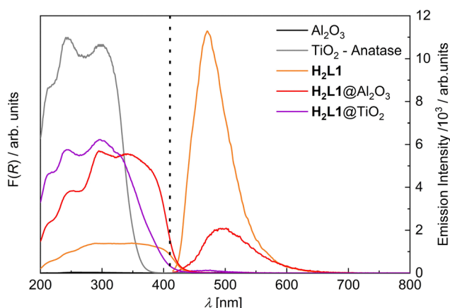
Fig. 4 Diffuse reflectance spectra (Kubelka–Munk analysis, left) and photoluminescence spectra (right) of bulk H 2 L1 , the neat substrates \text{TiO}_2 and \text{Al}_2\text{O}_3 , and the hybrid materials. Dashed line represents the excitation wavelength of 410 nm for the PL experiments.
