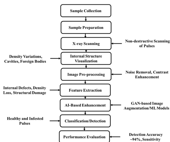
Fig. 9 X-ray imaging technique for pulse adulteration detection.
