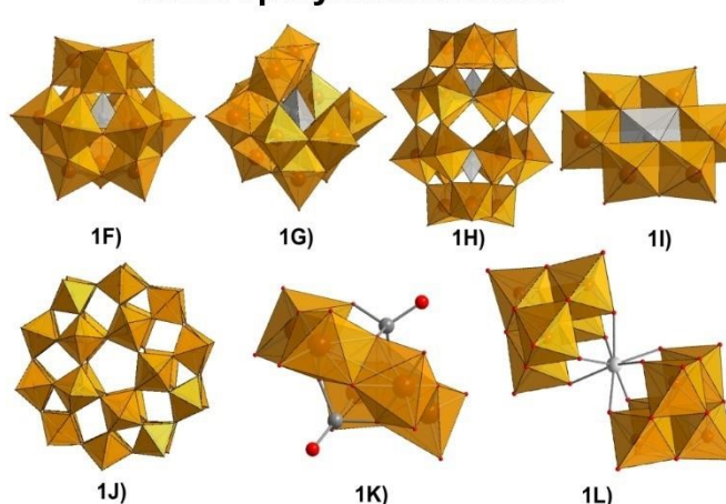
Figure 2. Structures of isopolyoxometalates and heteropolyoxometalates: 1A) Lindqvist ( [Mo_6O_{19}]^{2-} ), 1B) heptamolybdate ( [Mo_7O_{24}]^{6-} ), 1C) octamolybdate ( [Mo_8O_{26}]^{4-} ), 1D) decatungstate ( [W_{10}O_{32}]^{4-} ), 1E) decavanadate ( [V_{10}O_{28}]^{6-} ), 1F) Keggin ( [XM_{12}O_{40}]^{n-} ), 1G) monolacunary Keggin ( [XM_{11}O_{39}]^{n-} ), 1H) Wells-Dawson ( [X_2M_{18}O_{62}]^{n-} ), 1I) Anderson-Evans ( [XM_6O_{24}]^{n-} ), 1J) Preyssler ( [MP_5M_{30}O_{110}]^{(15-n)-} ), 1K) Strandberg ( [X_2Mo^V_5O_{23}]^{n-} ), and 1L) Weakley ( [M^{III}(M^{VI}_5O_{18})_2]^{n-} ). Color legend: orange = M (either Mo^VI , W^VI or V^V ), blue = Mo^VI , purple = W^VI , yellow = V^V , gray = X (heteroion), white = M^{III} , and red = oxygen.
