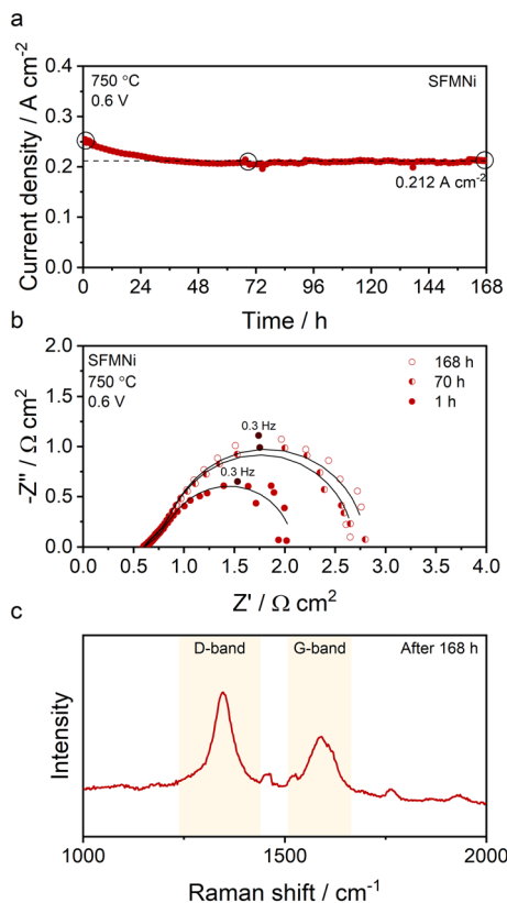
Fig. 6 Long-term stability of the SFMNi fuel electrode in an ethanol-steam atmosphere (2.6% EtOH–10.4% H 2 O–N 2 ) at 0.6 V and 750 °C. (a) Potentiostatic performance at 0.6 V over 7 days, (b) corresponding Nyquist plots recorded after 1 h, 70 h, and 168 h, illustrating the evolution and stability of cell resistance contributions and (c) Raman spectrum of the spent cell after 168 h demonstrating the presence of carbon deposits.
