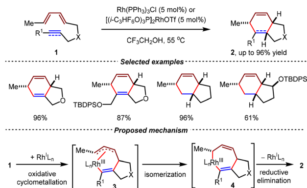
Scheme 4 Rhodium(I)-catalyzed intramolecular [4+2] cycloadditions of diene-yne and trienes.
