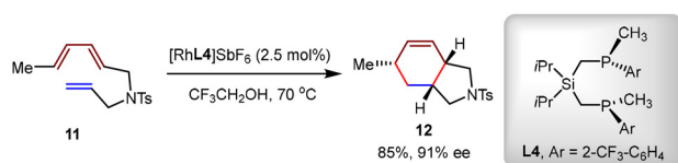
Scheme 7 Rhodium(i)-catalyzed asymmetric intramolecular [4+2] cycloaddition of the nitrogen-tethered triene.
