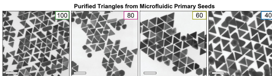
Fig. 8 STEM images of purified gold nanotriangles derived from the m-PS sample. Labels indicate the utilized volume of intermediate seeds (μL). Scale bars are 100 nm. Reprinted from ref. 31 with permission from E. Podlesnaia, P. G. Inangha, J. Vesenska, M. Seyring, H.-J. Hempel, M. Rettenmayr, A. Csáki and Wolfgang Fritzsche, Small , 2023, 19 , 2204810. Copyright 2023 John Wiley & Sons, Inc.
