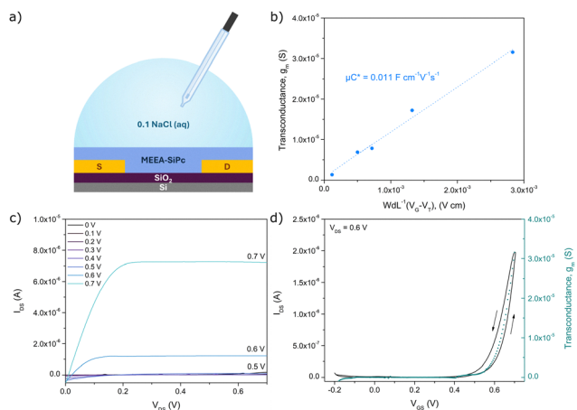
Fig. 5 (a) Schematic of the MEEA-SiPc OEET. (b) Determination of \mu C^* from the plot of g_m vs. WdL^{-1}(V_{GS} - V_T) . Characteristic (c) output and (d) transfer curves of MEEA-SiPc OEETs in 0.1 M NaCl with W = 10\,000 \mu m, L = 2.5 \mu m.
