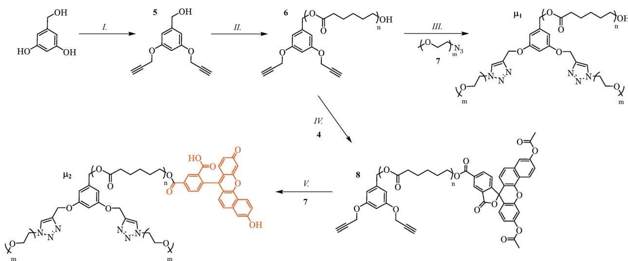
Scheme 4 Synthesis of miktoarm polymers μ 1 (unlabelled PEG 2 –PCL) and μ 2 (fluorescent PEG 2 –PCL–SNAFL). (I) Propargyl bromide, K 2 CO 3 , 18-crown[6], acetone, 60 °C, 18 h. (II) \epsilon -Caprolactone, tin(II) ethyl hexanoate, toluene, 110 °C, 18 h. (III) mPEG 2000 -N 3 ( 7 ), CuBr, N,N'-PMDETA, DMF, 40 °C, 24 h. (IV) SNAFL-diacetate ( 4 ), DCC/DMAP, DCM, 0 °C – RT, 48 h. (V) CuBr, N,N'-PMDETA, DMF, 40 °C, 24 h.
