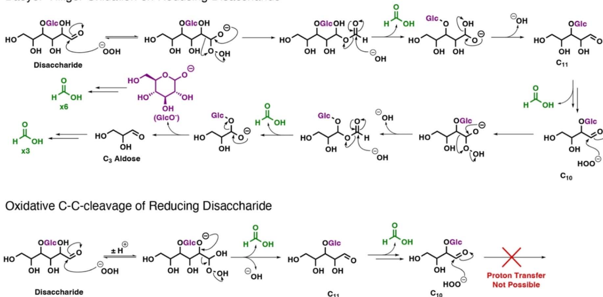
Scheme 3 Plausible mechanisms in the degradation of cellobiose in the presence of a hydroperoxyl anion. The absence of C 10 disaccharide and the rapid and full conversion to formate argue for a central role of Baeyer–Villiger oxidation.
