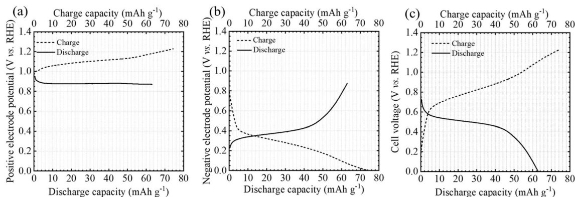
Fig. 2 Charging/discharging curves of the SSAB-PPNQ cell measured at a current density of 0.23 \text{ mA cm}^{-2} : (a) positive electrode potential, (b) negative electrode potential, and (c) cell voltage.
