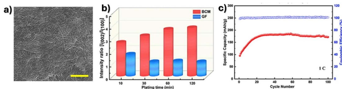
Fig. 5 (a) SEM images of a cycled bacterial cellulose based separator; (b) intensity ratio of crystal planes from Zn plating and (c) stability of the battery at 1C. Reproduced from ref. 119, with permission. Copyright 2022, Cell Press.
