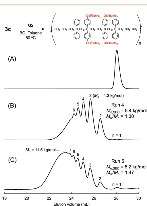
Fig. 3 SEC curves of 3c (A), after ADMET polymerization of 3c with BQ in toluene at 60 °C for 24 h (B) and for 48 h (C).
