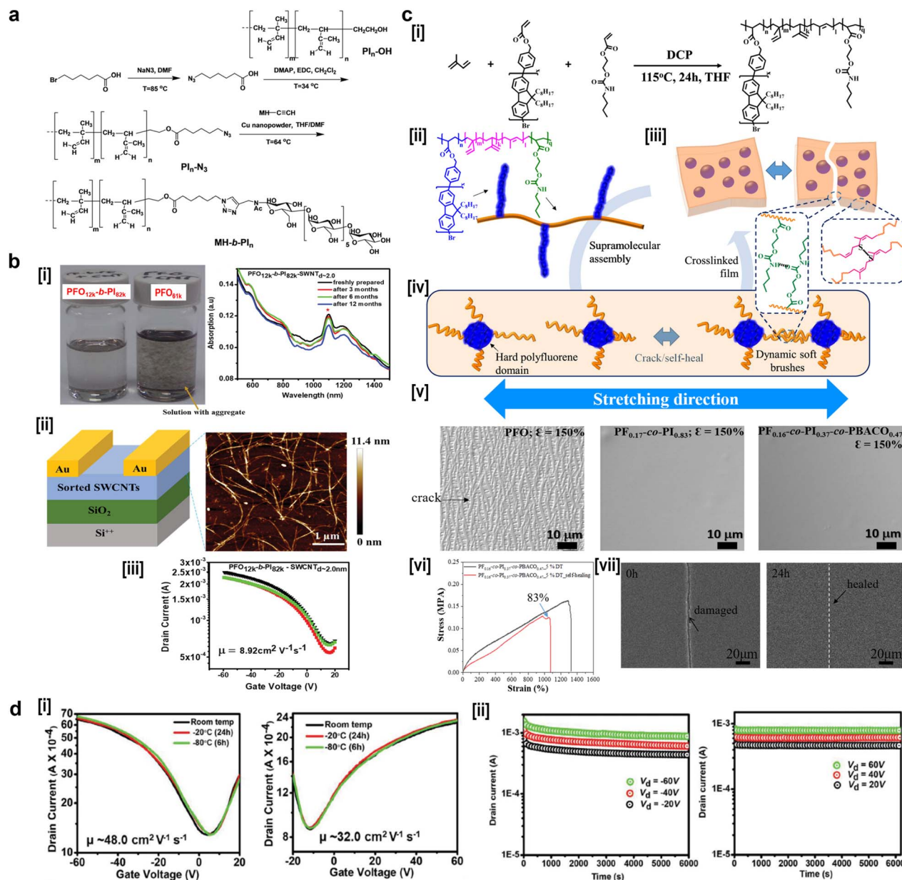
Fig. 8 (a) The synthesis routes of \text{MH-b-PI}_n block copolymers for stretchable resistive memory device application. (b) SWCNTs-thin film transistor fabrication: (i) stability and dispersion study based on photograph image and UV-spectra, (ii) schematic of BGTC transistor configuration and AFM image of SWCNTs sorted by \text{PFO}_{12K}\text{-b-PI}_{82K} , and (iii) I_D\text{-}V_G transfer curve of the device using \text{PFO}_{12K}\text{-b-PI}_{82K} -dispersed sc-SWCNTs (diameter \leq 2.0 nm) as the semiconducting layer. (c) Molecular design of the intrinsically elastic and self-healing luminescent \text{PF}_x\text{-co-PI}_y\text{-co-PBACO}_z : (i) synthetic scheme; (ii) branched copolymer with soft PI-co-PBACO backbone (blue) and rigid PF branches (orange); (iii) self-assembled into a two-phase nanostructure; (iv) elasticity tuning via DT cross-linking (gray spheres) and hydrogen bonding (dotted lines), (v) OM images of the PF, \text{PF}_{0.17}\text{-co-PI}_{0.83} , and \text{PF}_{0.16}\text{-co-PI}_{0.37}\text{-co-PBACO}_{0.47} thin films under 150% strain, and (vi) investigation RT self-healing performance of the \text{PF}_{0.16}\text{-co-PI}_{0.37}\text{-co-PBACO}_{0.47} film based on tensile test and SEM images before (0 h) and after (24 h) self-healing. (d) The (i) ( I_D\text{-}V_G ) transfer curves and (ii) retention stability of p-type and n-type \text{PF}_{0.16}\text{-co-PI}_{0.36}\text{-co-PBACO}_{0.48} -sc-SWCNTs respectively, where the retention tests were performed at gate voltages of \pm 60 V. Reprinted with permission from ref. 19. copyright 2017 John Wiley & Sons., ref. 134 copyright 2021 John Wiley & Sons, ref. 62 copyright 2022 American Chemical Society, ref. 139 copyright 2022 John Wiley & Sons.
