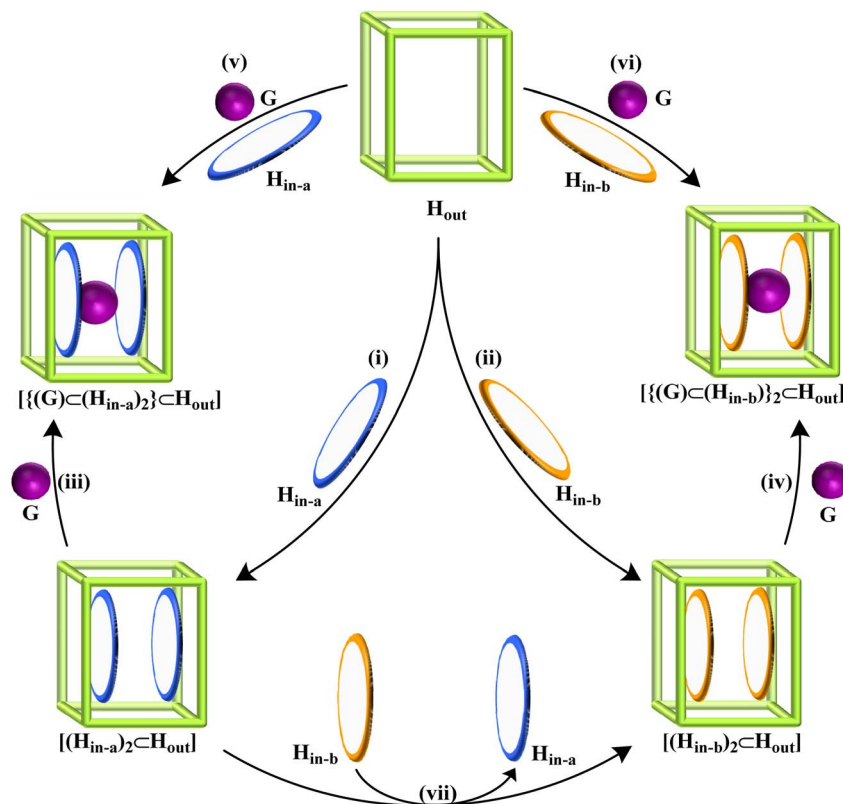
Fig. 1 Conceptualizing the synthesis of assemblies of (i and ii) [(H_{in})_2 \subset (H_{out})] and (iii–vi) \{(G) \subset (H_{in})_2\} \subset (H_{out}) type molecules. (vii) H_{in} exchange reaction showing selective inclusion of one type of H_{in} over another type of H_{in} by H_{out} .
