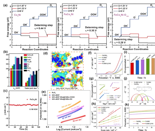
Fig. 5 (a) The free-energy diagrams of \text{Co}_2\text{Ni-MOF-74} , \text{FeCo}_2\text{Ni-MOF-74} and \text{FeCo}_2\text{Ni-Ox} . (b) Comparison of the Tafel slope and overpotential of precious metal oxides and the MOF materials in this work. (c) The stability measurements for \text{FeCo}_2\text{Ni-MOF-74} . (d) The difference charge density of catalysts. Yellow indicates a decrease in electron density, while blue signifies an increase. (e) Tafel plots of catalysts. (f–k) The electrochemical performance of the Ni-BDC@NIS comparison sample. 76
