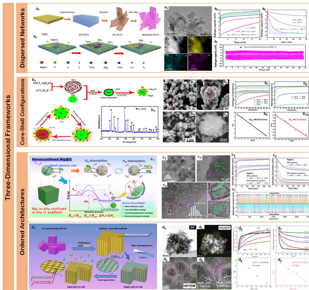
Fig. 11 (a1) Schematic view of MXene preparation from the MAX phase by Al layers selective etching, exfoliation of the 2D structure (2D-TiVCT x ); (a2) and formation of the 3D delaminated (3D-TiVCT x ) structure and composite with MgH 2 nanoparticles; structural and morphology studies of MgH 2 @3D-TiVCT x : (a3) TEM micrographs, and (a4) HAADF and STEM-EDS mapping after cyclic performance. (a5 and a6) Hydrogenation and dehydrogenation kinetic performance at different temperatures, while (a7) sorption cyclic performance of MgH 2 @3D-TiVCT x at 250 °C. 158 (b1) Schematic diagram of the fabrication of the Mg–MgS–Mg 2 Ni–Ni nanocomposite and its first activation process at 673 K; (b2) XRD pattern of the NiS flowerlike particles; SEM (b3) and high magnification SEM (b4) images of the NiS flowerlike particles; (b5) SEM, (b6) high magnification SEM images of the nanocomposite; hydrogen absorption curves under 4 MPa hydrogen pressure (b7), desorption curves under 100 Pa (b8), plots of \ln -k vs. 1000/T for the hydrogenation (b9) and dehydrogenation (b10) of Mg–MgS–Mg 2 Ni–Ni nanocomposite. 159 (c1) Schematic diagram of hydrogen absorption and desorption reaction mechanism of the Mg@C nanocomposites; (c2 and c3) TEM images of MgBu 2 (inset: the particle size distribution histogram of MgBu 2 ) and MgBu 2 @ZIF-8; HRTEM image (c4) (inset: the particle size distribution histogram of Mg); isothermal hydrogenation and dehydrogenation cycle curves of the Mg@C-3 (c5); isothermal hydrogenation curves (c6) and dehydrogenation curves (c7) of the Mg@C-3 after synthesis and after 30 days in air. 160 (d1) Schematic illustrations of the nanoconfinement process for the synthesis of MgH 2 @CoS-NBs composite; typical bright field TEM image (d2); HAADF image (d3) and HRTEM micrographs (d4 and d5) for the MgH 2 @CoS-NBs composite, subjected to several H-cycles; isothermal hydriding (d6) and dehydriding (d7) profiles of Mg@CoS-NBs composite, and the corresponding \ln -k vs. 1000/T plots for determining the activation energy of hydrogenation (d8) and dehydrogenation (d9). 161
