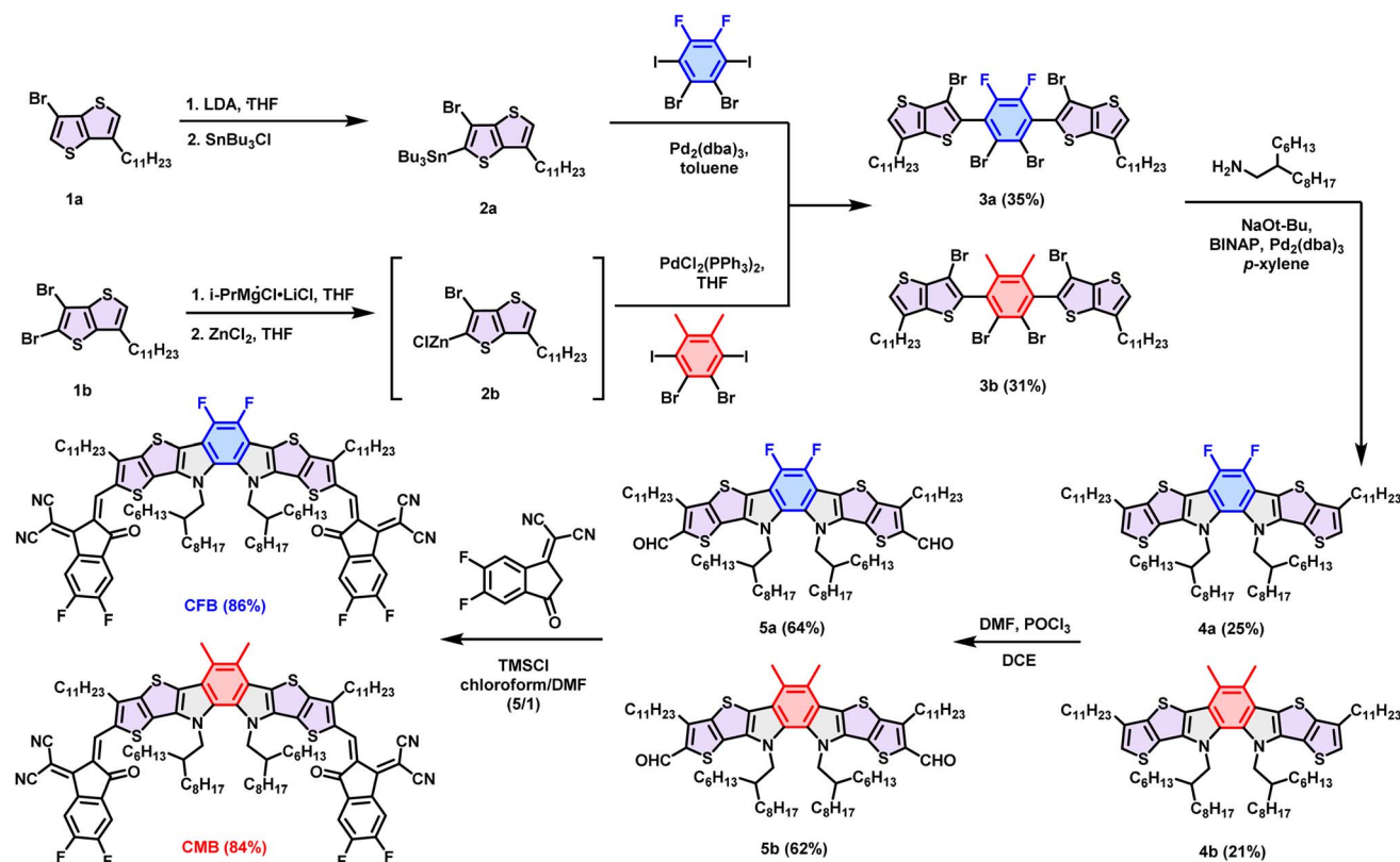
Scheme 1 Synthetic routes for o-BDP-based CFB and CMB.
