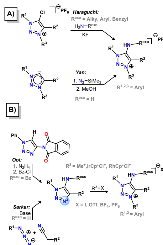
Scheme 2 Hitherto reported synthetic routes to 5-amino-1,2,3-triazolium salts. A) Amine-functionalisation of 1,2,3-triazolium salts. B) Construction of 5-amino-1,2,3-triazolium salts followed by quaternisation of N3.
