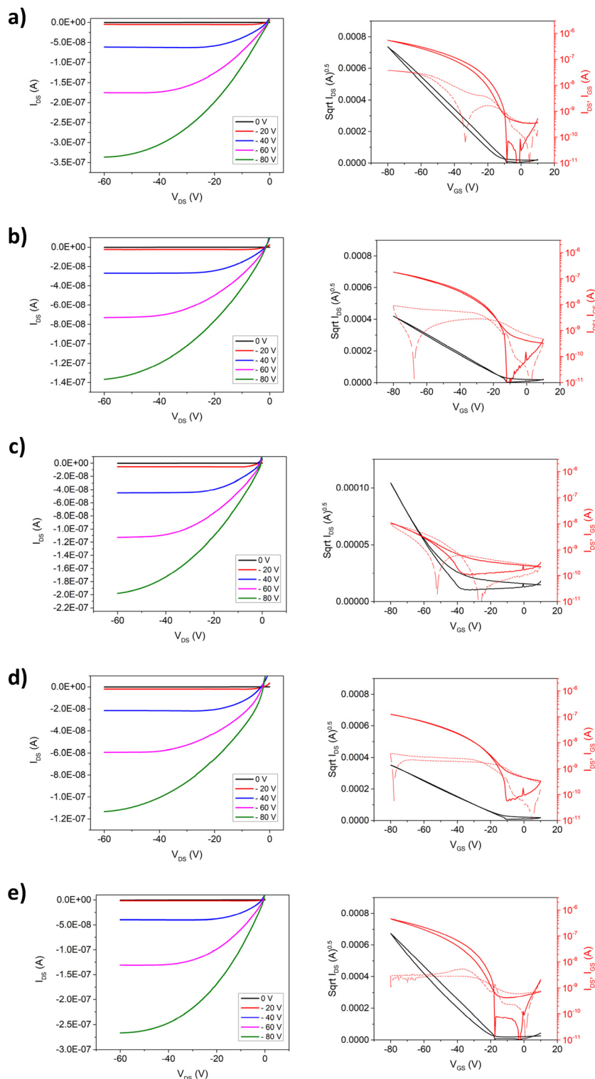
Fig. 2 Representative output characteristics (left) and transfer curves (right) of PI[(iITT)(C n C x C y )(C 12 )] series; (a) PI[(iITT)(C 1 C 10 C 12 )(C 12 )], (b) PI[(iITT)(C 1 C 10 C 10 )(C 12 )], (c) PI[(iITT)(C 2 C 10 C 10 )(C 12 )], (d) PI[(iITT)(C 3 C 10 C 10 )(C 12 )], and (e) PI[(iITT)(C 4 C 10 C 10 )(C 12 )]. All measurements were performed on thin films prepared via spin coating of a chlorobenzene solution of selected polymer (5 mg ml -1 ). All OFET devices were fabricated after thermal annealing for 1 hour at 150 °C, V DS = -80 V.
