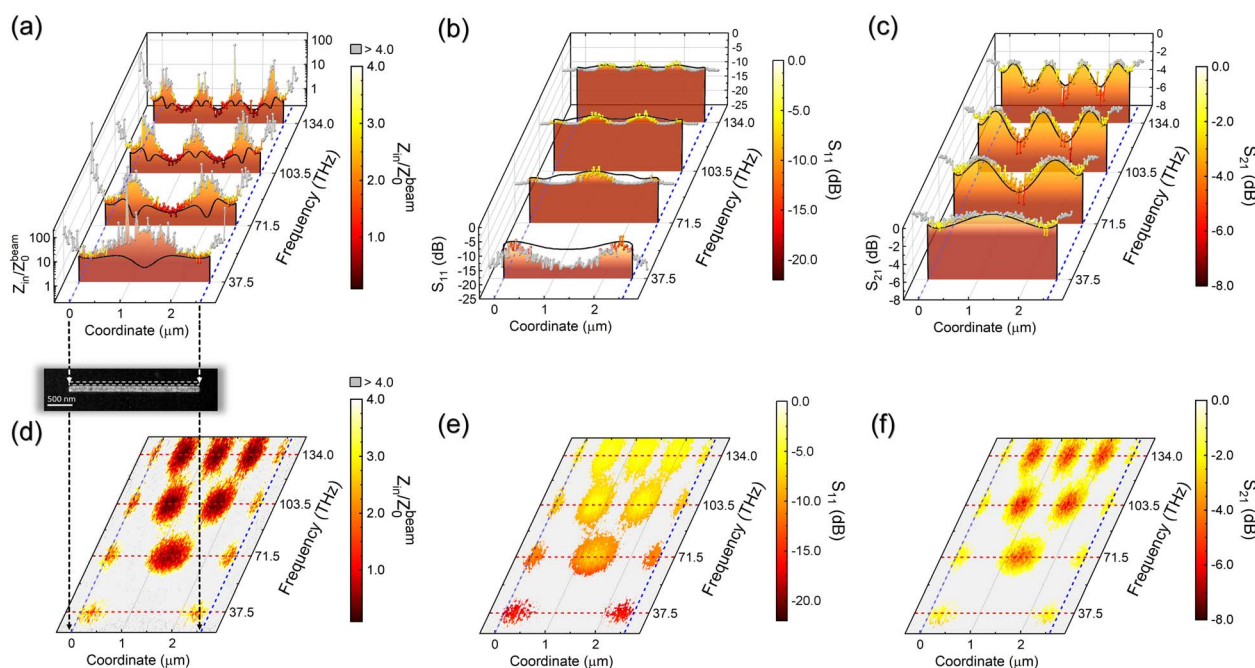
Fig. 7 The profiles of experimentally characterized microwave parameters (color plots) at the first four resonances of the plasmonic dipole: input impedance Z_{in} (a) relative to the beam characteristic impedance Z_0^{beam} , S_{11} (b), and S_{21} (c) parameters. The microwave parameters obtained through full-wave simulations are shown alongside as black curves. Regions of considerable discrepancy between experimentally characterized and simulated impedances are depicted as gray points in (a–c), assisting in identifying areas with minimal uncertainty, illustrated as color spots in the maps (d–f) for the above-shown parameters. The arrows denote the positions of the edges of the investigated dipole. The dashed area in the dipole topography image (shown below (a)) highlights the region from which the microwave parameter profiles were extracted.
