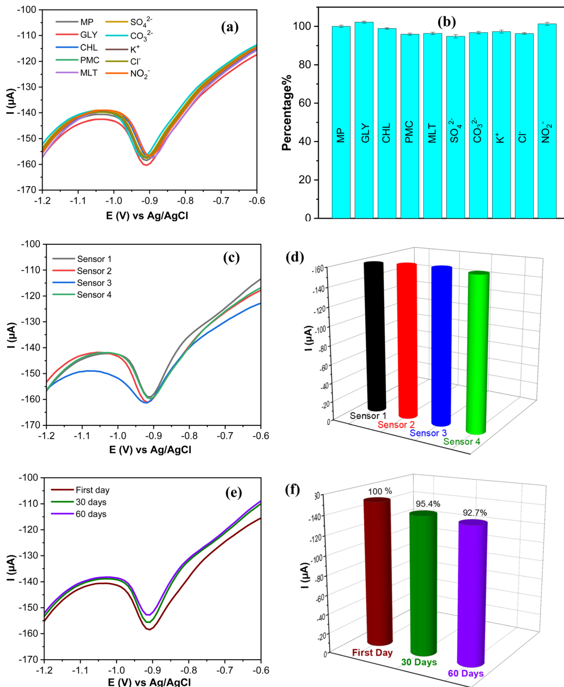
Fig. 13 (a) SWV curves of 20 \mu\text{mol L}^{-1} PM on AgNPs@GO/IL@SPCE (E5) in the presence other interfering compounds. (b) Bare diagram of the current percentage change of PM reduction in the presence of interfering species. (c) SWV response of four AgNPs@GO/IL@SPCE (E5) electrodes towards 20 \mu\text{mol L}^{-1} PM. (d) Bare diagram evaluation of the reproducibility study. (e) SWV response of AgNPs@GO/IL@SPCE (E5) over storage time. (f) Bare diagram evaluation of the long-term stability study. Note: geometric area of the working electrode: 7 mm 2 .
