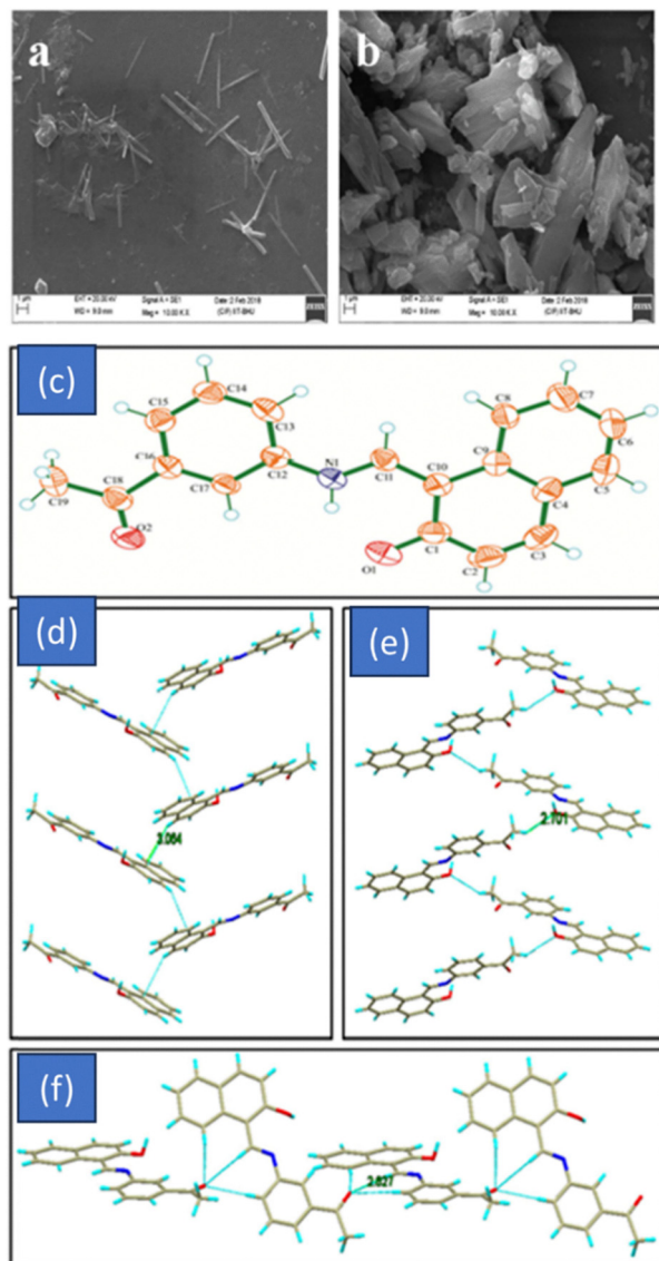
Fig. 22 SEM image of HL 9 (20 μM) showing aggregates in different acetonitrile–water mixtures (a) f_w = 70\% and (b) f_w = 90\% . (a) ORTEP diagram of HL 9 with ellipsoid of 30% probability. Crystal packing in the HL 9 molecule (b) showing C–H... \pi interactions and (c) and (d) showing C–H...O interactions; reproduced from ref. 25 with permission from Elsevier, Copyright 2019.
