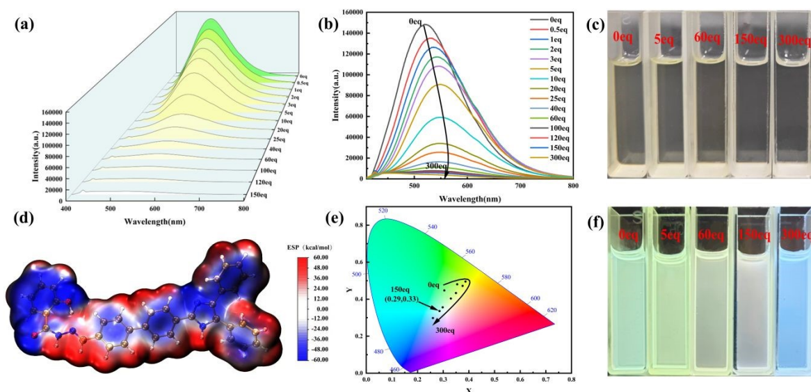
Figure 4. (a) Fluorescence color evolution of Q in DMSO solution with varying \text{H}^+ equivalents. (b) Emission spectra of Q ( 1 \times 10^{-3} M in DMSO) as a function of \text{H}^+ concentration (0–300 eq.). (c) Visible-light photographs showing the color progression of Q in DMSO with increasing \text{H}^+ content. (d) Simulated electrostatic potential (ESP) distribution of Q. (e) Corresponding CIE chromaticity diagram for (b). (f) Corresponding UV-illuminated (422 nm) photographs demonstrating the fluorescence color transition for (c).
