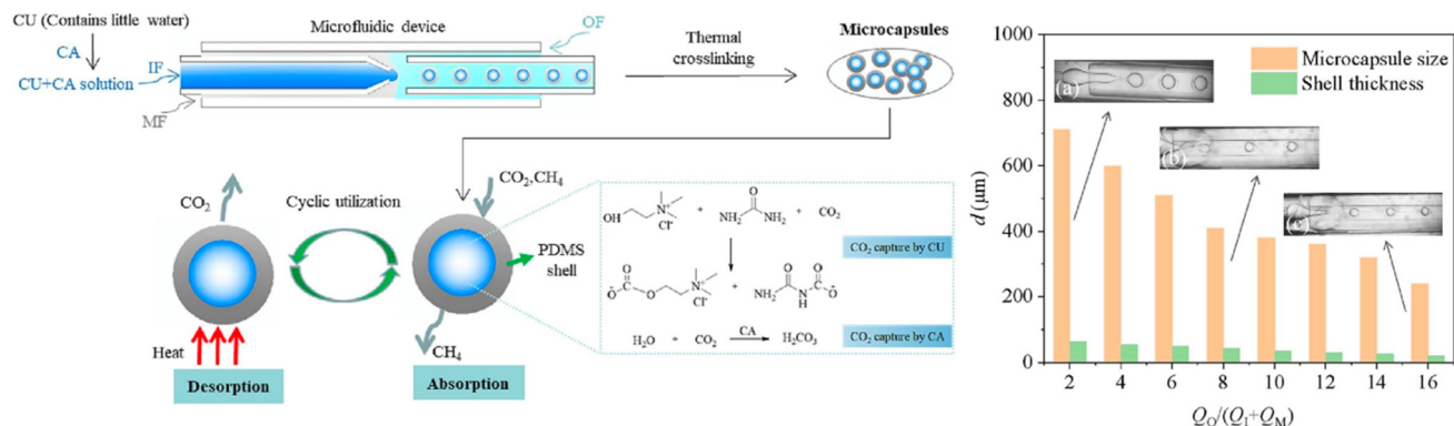
Fig. 3 [Left] Schematic diagram of the flow-focusing microchannel, encapsulating DES and CA. IF – inner fluid; MF – middle fluid; OF – outer fluid. [Right] Effect of the flow rates on the microcapsule size and shell thickness in a 3D glass-capillary microfluidic device (in the graph, “d” as a function of Q_O/(Q_I + Q_M) – flow rate of inner fluid; Q_M – flow rate of middle fluid; Q_O – flow rate of outer fluid: figures (a)–(c) show actual experimental images of microcapsules with varying sizes and shell thicknesses). 31
