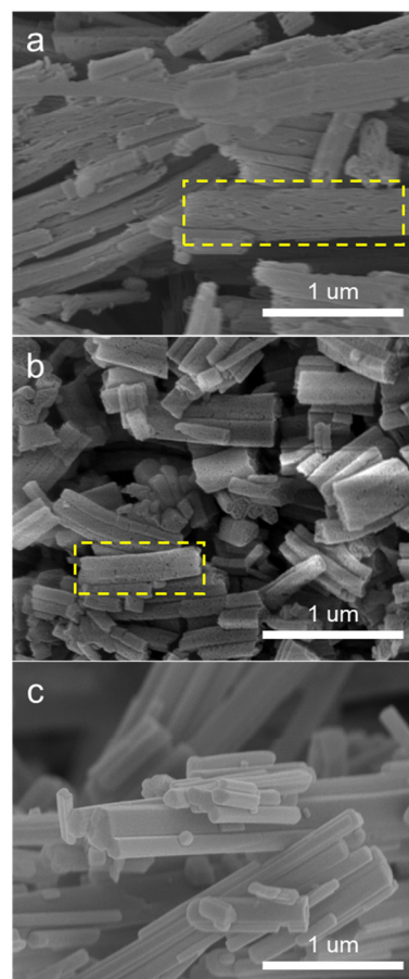
Fig. 7 SEM images of (a) bare Mg 2 (dobpdc), (b) BPEI(30)-Mg 2 (dobpdc), and (c) TEPA(50)-Mg 2 (dobpdc) after 5 humid adsorption/desorption cycles. Adsorption and desorption conditions were 30 °C and 50% RH for 2 h with 400 ppm CO 2 /N 2 and 80 °C and dry N 2 for 2 h, respectively. Perforation (yellow box) on the crystal surfaces of the (a) bare Mg 2 (dobpdc) and (b) BPEI(30)-Mg 2 (dobpdc) is notable.
