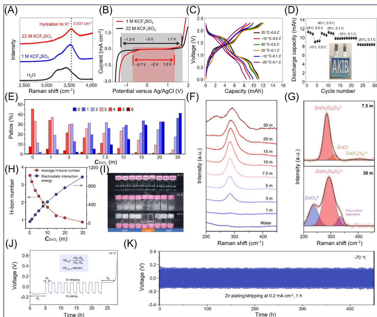
Figure 4. (A) Raman spectra of different concentrations of KCF 3 SO 3 electrolyte. (B) Electrochemical window for 1 M and 22 M KCF 3 SO 3 electrolytes. (C) Typical charge/discharge curves of KFeMnHCF-3565//22 M KCF 3 SO 3 /PTCDI pouch batteries at different rates and
