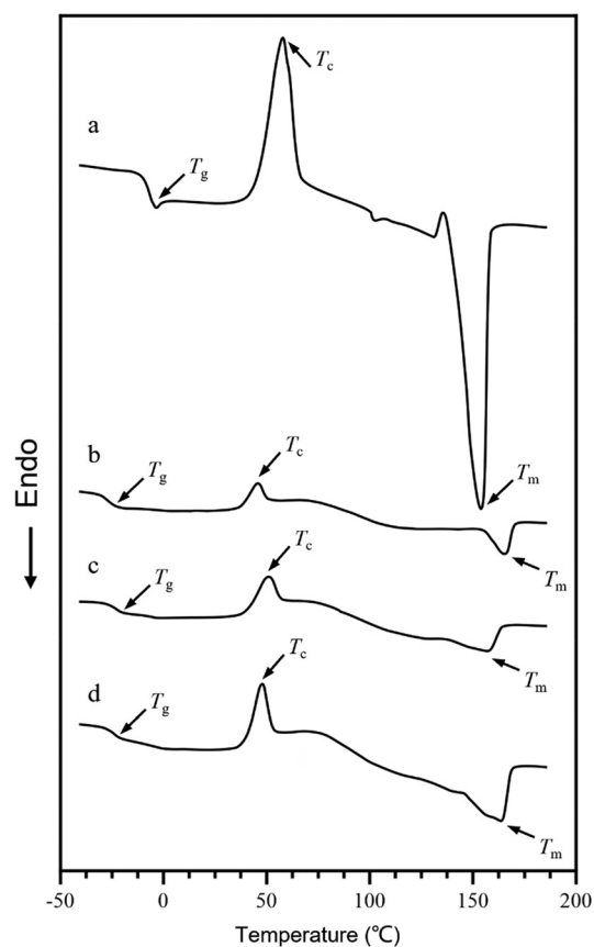
Fig. 8 Differential scanning calorimetry (DSC) thermographs of P3HB3H9Od containing different proportions of P3H9Od produced by H. bluephagenesis TXY32E. (a) P3HB. (b) P(3HB- co -5 mol% 3H9Od). (c) P(3HB- co -7.5 mol% 3H9Od). (d) P(3HB- co -10 mol% 3H9Od).
