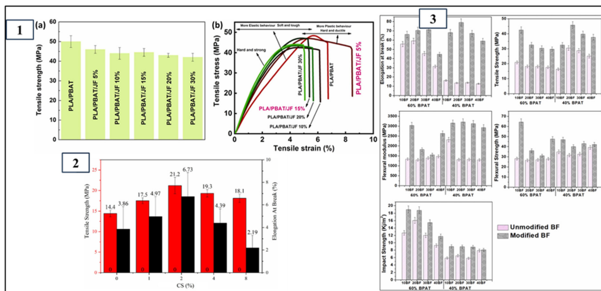
Fig. 6 Effects of different natural fiber on the mechanical properties of biodegradable blend composite. (1) (a) tensile strength of PLA/PBAT with different jute fiber amounts, (b) tensile stress of PLA/PBAT with different jute fiber amounts. (2) tensile strength and elongation at break of cotton stalk-reinforced PLA/PBAT composite, (3) mechanical properties of bamboo fiber-reinforced PLA/PBAT (elongation at break, tensile strength, flexural strength, flexural modulus and notched Izod impact strength). (1) was reproduced from ref. 187 with permission from Elsevier; copyright 2025, (2) was reproduced from ref. 186, with permission from Wiley, copyright 2025, (3) was reproduced from ref. 55, with permission from Elsevier, copyright 2025.
