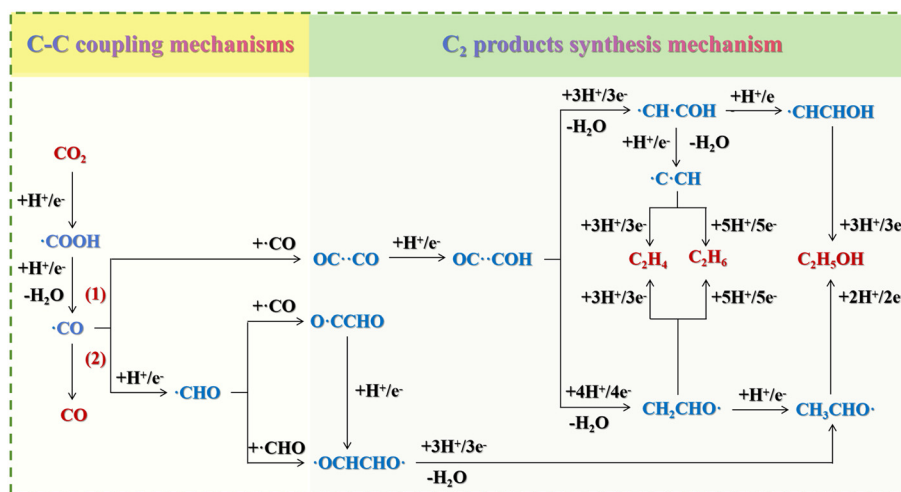
Fig. 6 Reaction pathways of CO 2 reduction to produce value-added C 2 chemicals (C 2 H 4 , C 2 H 6 , and C 2 H 5 OH) via electrocatalysis by adding (1) \cdot\text{CO} before H + /e - and (2) H + /e - before \cdot\text{CO} .
