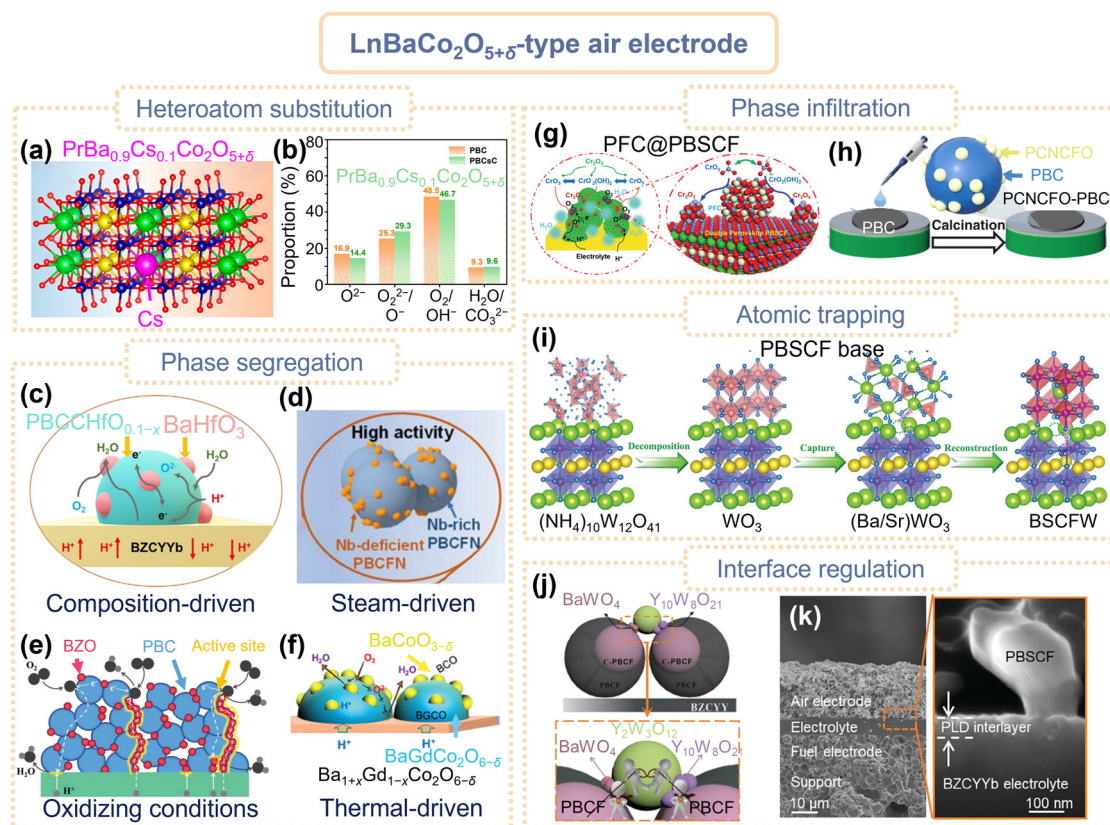
Fig. 10 Recent advances in \text{LnBaCo}_2\text{O}_{5+\delta} -type air electrode materials. (a) Structure of PBCsC, (b) comparisons of different oxygen species contents of PBS and PBCsC. Reproduced with permission. 226 Copyright 2023, American Chemical Society. (c) Schematic of Hf-doped PBCCHf 0.1 . Reproduced with permission. 229 Copyright 2024, Elsevier. (d) Schematic of PBCFN. Reproduced with permission. 230 Copyright 2022, Wiley-VCH. (e) Schematic of BZO@PBC. Reproduced with permission. 231 Copyright 2022, Wiley-VCH. (f) Schematic of BGCO–BCO hybrid catalyst. Reproduced with permission. 232 Copyright 2024, Wiley-VCH. (g) Schematic of PFC@PBSCF in the presence of contaminants (Cr and steam). Reproduced with permission. 234 Copyright 2022, Wiley-VCH. (h) Schematic for the fabrication procedures of PCNCFO–PBC. Reproduced with permission. 235 Copyright 2024, Wiley-VCH. (i) Structural evolution during reverse atom capture process. Reproduced with permission. 150 Copyright 2024, Wiley-VCH. (j) Mechanism underlying the thermo-mechanical enhancement of TEC gradient formation. Reproduced with permission. 382 Copyright 2024, Wiley-VCH. (k) Cross-sectional SEM image of PBSCF/BZCYYb composite interlayer. Reproduced with permission. 236 Copyright 2024, Wiley-VCH.
